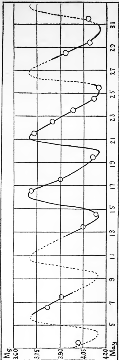
Figure 24 SINGLE LIGHT CURVES OF \delta CEPHEI
