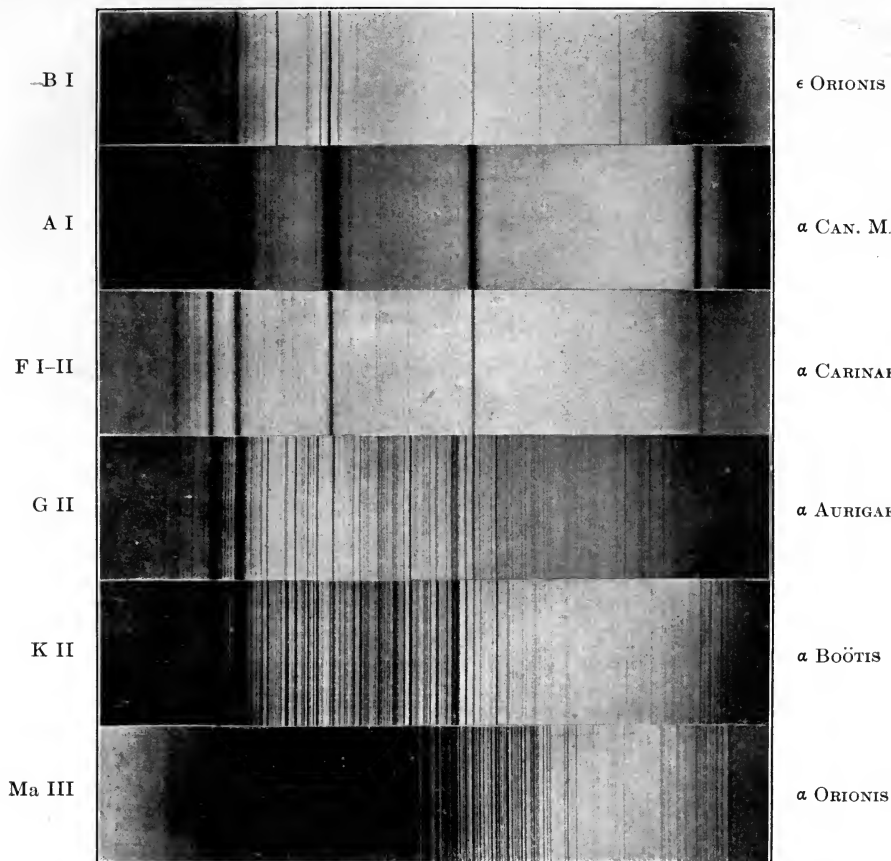
Plate XIII TYPICAL SPECTRA
