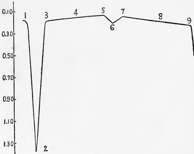
Figure 29. Diagram I THE LIGHT CURVE
