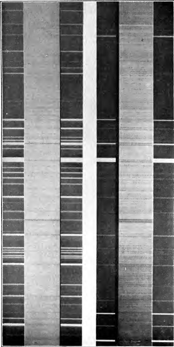
Plate X SPECTRA OF \zeta URSAE MAJORIS
