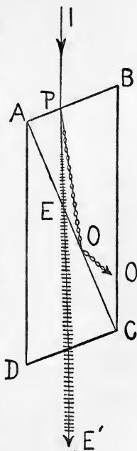
Figure 17 THE NICOL'S PRISM
