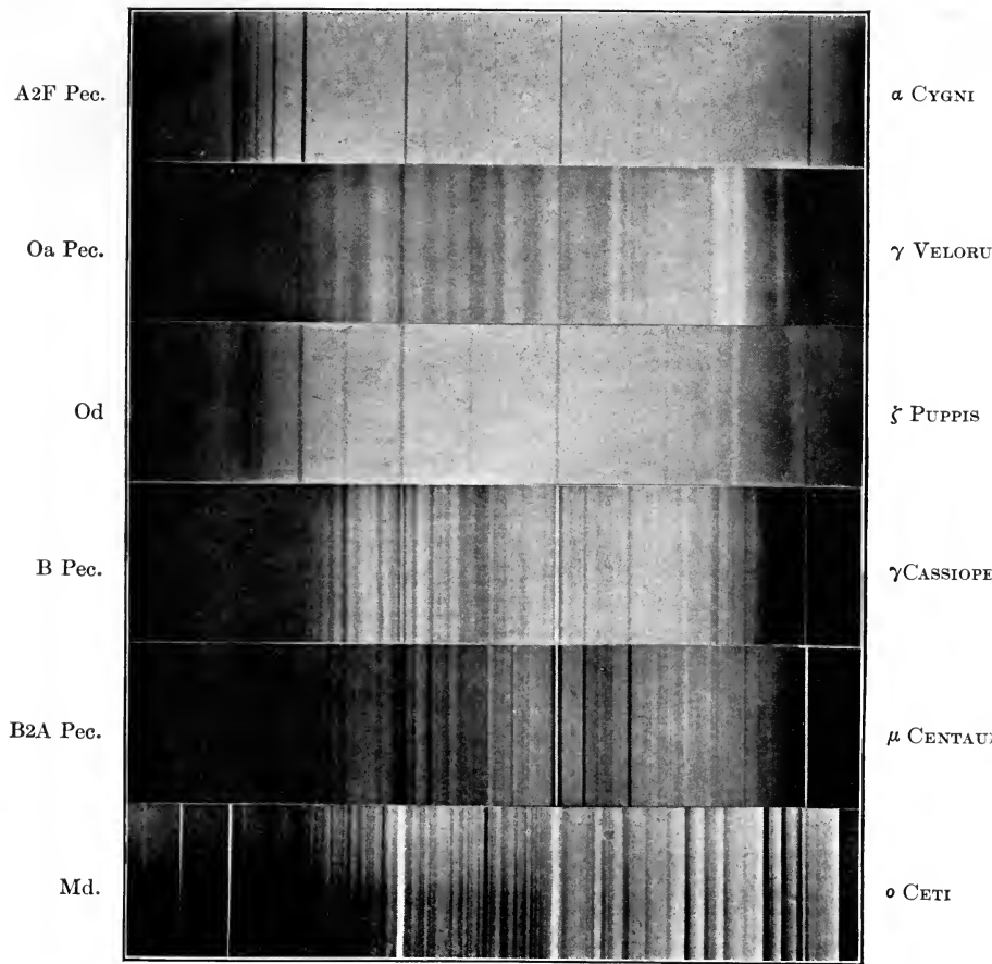
Plate XIV PECULIAR SPECTRA
