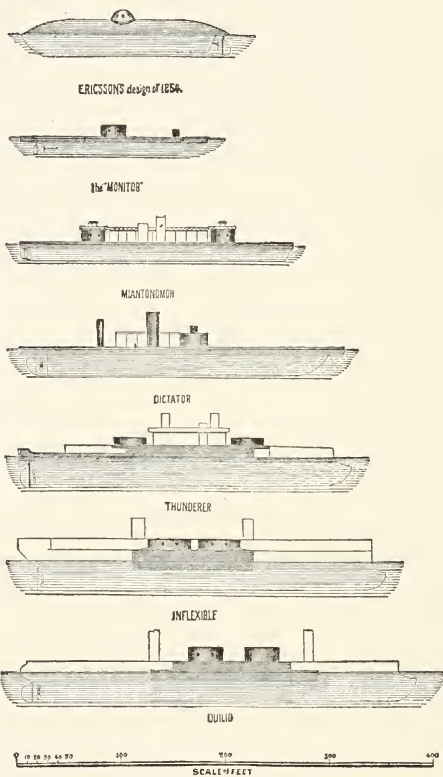
Development of the Monitor Idea.
