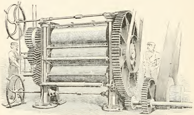
Calenders Heated Internally by Steam, for Spreading India Rubber into Sneets or upon Cloth, called the "Chaffee Machine."
