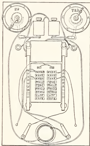
Vote Recorder—Edison's First Patented Invention.
