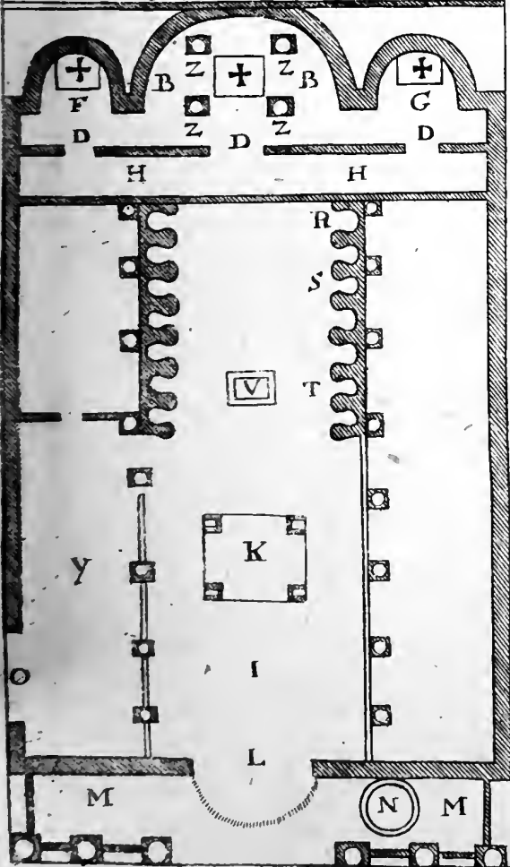
Ichnographia Jacobi Goar
