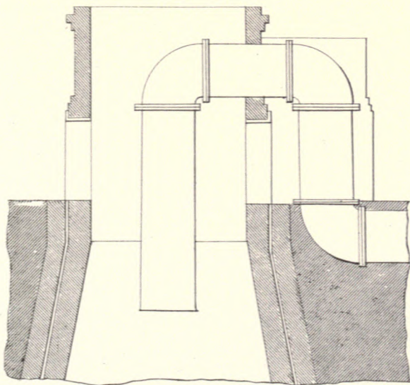
MODES OF COLLECTING FURNACE GASES
