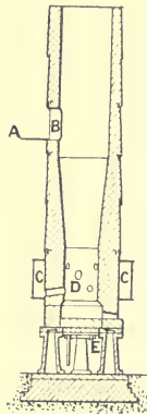
FIG. 20.—Foundry Cupola.
