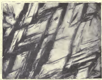
FIG. 68.—Austenite and Martensite.
