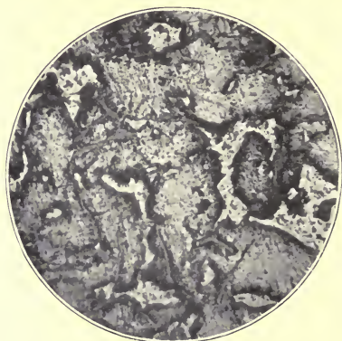
FIG. 71.—Cast Iron with Phosphide Eutectic.
