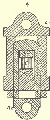
FIG. 61.— Shackles.
