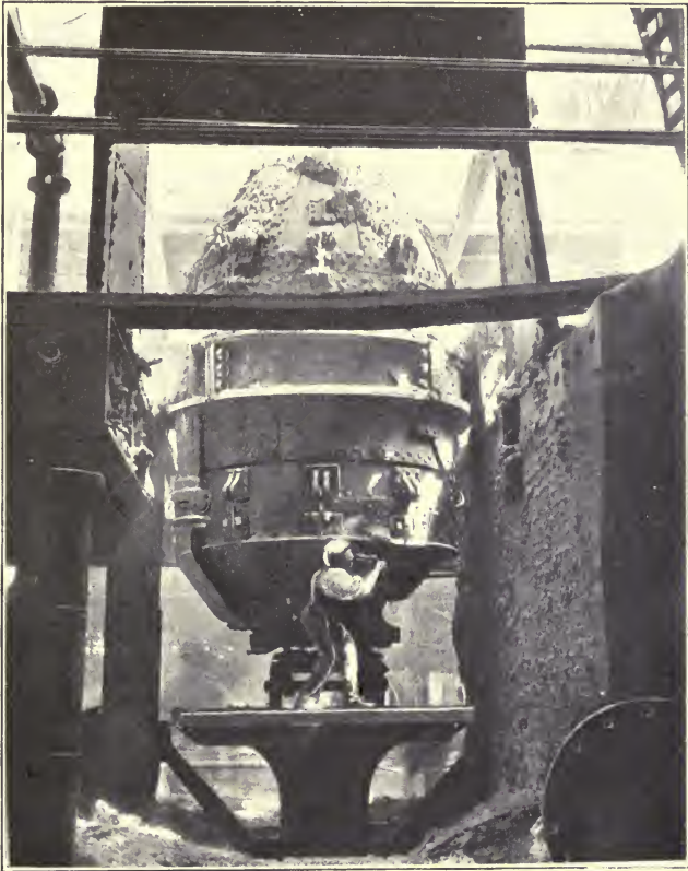
FIG. 34.—Bessemer Converter in Position.
