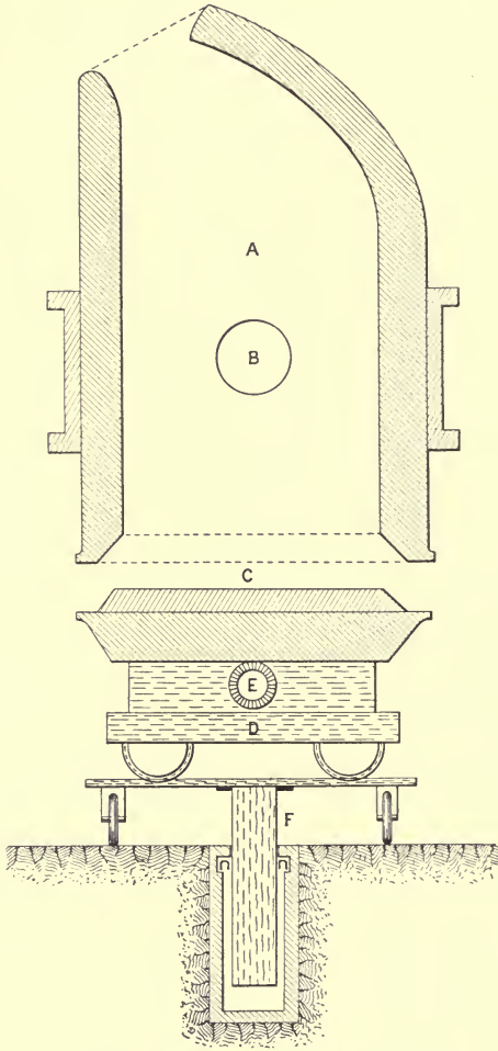
FIG. 30.—Eccentric Converter.
