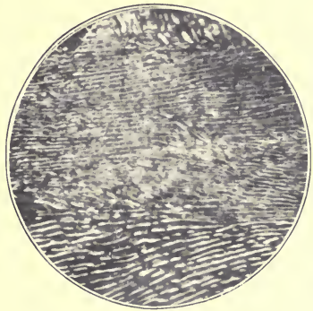
FIG. 67.—Pearlite (Stead).
