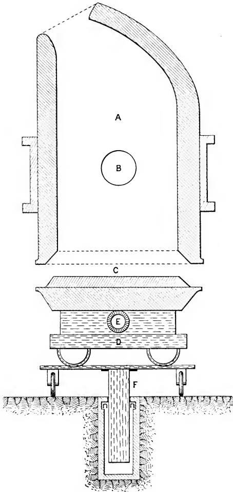
FIG. 30.—Eccentric Converter.
