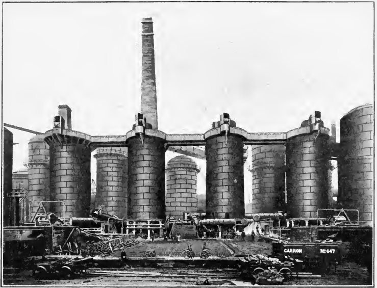
A Scotch Blast Furnace Plant, Carron Works.
