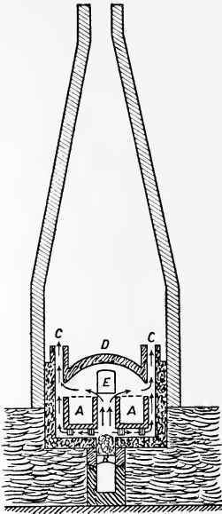
FIG. 25. -- Cementation Furnace.
