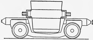
FIG. 31.—Tilting Ladle.
