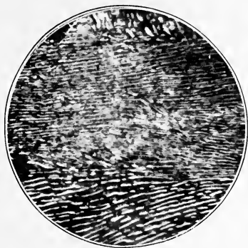
FIG. 67.—Pearlite (Stead).
