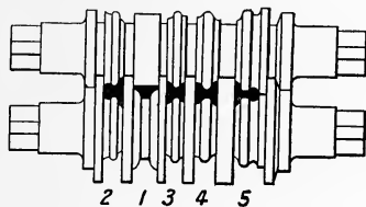
FIG. 55.—Rail Rolls.
