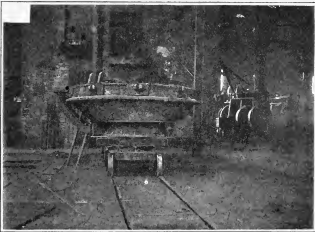
FIG. 35.—Converter Bottom in Repairing Shop.
