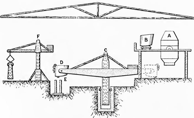
FIG. 33.—Converter and Cranes in Bessemer Shop.
