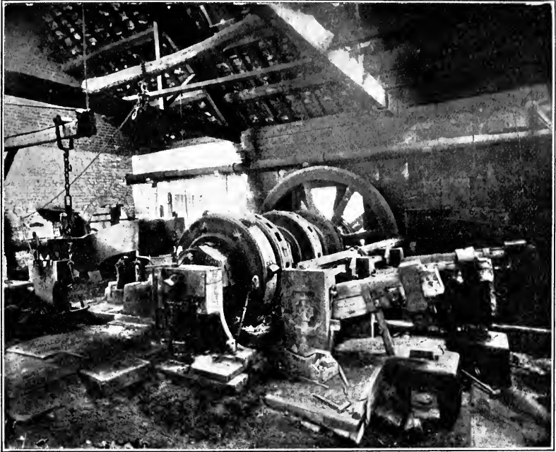
FIG. 46.—Interior of the Clay Wheel Forge showing Tilt Hammers driven by Water Power.
