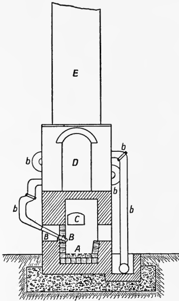
FIG. 28.—Styrian Open Hearth.
