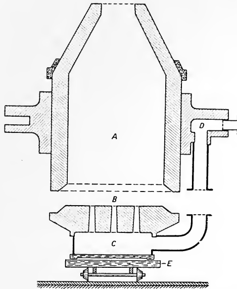
FIG. 29.—Concentric Converter.
