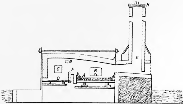
FIG. 22.—Puddling Furnace (vertical section).
