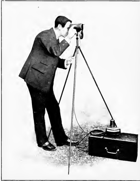
FIG. 80.—Radiation Pyrometer.
