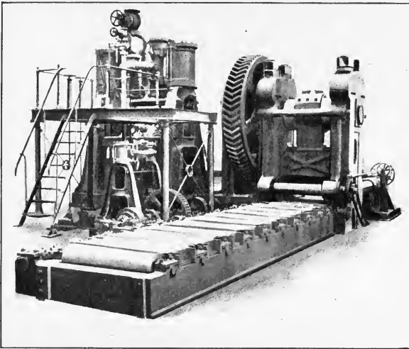
FIG. 54.—Blooming Shears.
