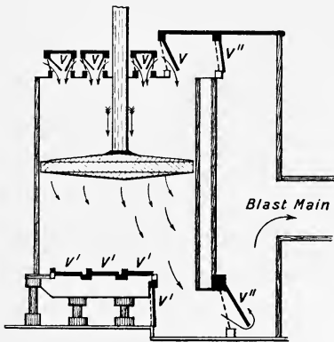
FIG. 15.—Blowing Cylinder.
