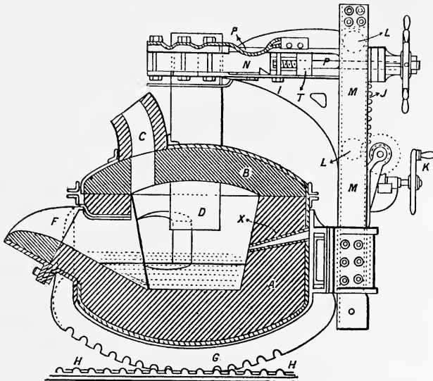
FIG. 82.—The Héroult Furnace.
