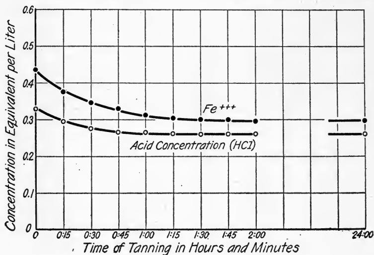
Curves Showing Absorption of Fe and HCl during Tanning
