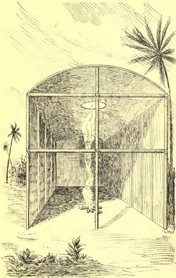
IROQUOIS HOUSE.
