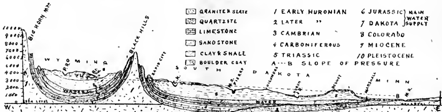
SECTION ILLUSTRATING THE ARTESIAN RESOURCES OF THE NORTHWEST IRRIGATION AGE
