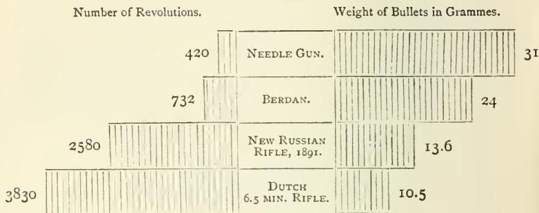
Rotation and Weight of Bullets of Various Rifles.
