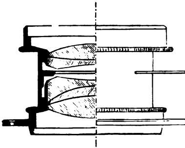
Fig. 98. Steinheil's neuer Antiplanet.
