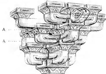
FIG. 72.—COMPOUND BRACKET.
