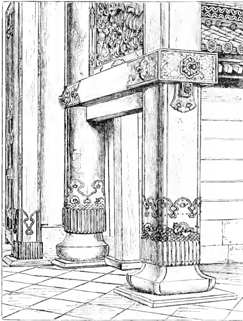
FIG. 44.—DETAILS OF EAST GATEWAY OF THE TEMPLE, NISHI-HONGWAN-JI, KIOTO.
