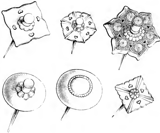
FIG. 36.—OLD NAILS FROM TEMPLE-DOORS IN NARA.
