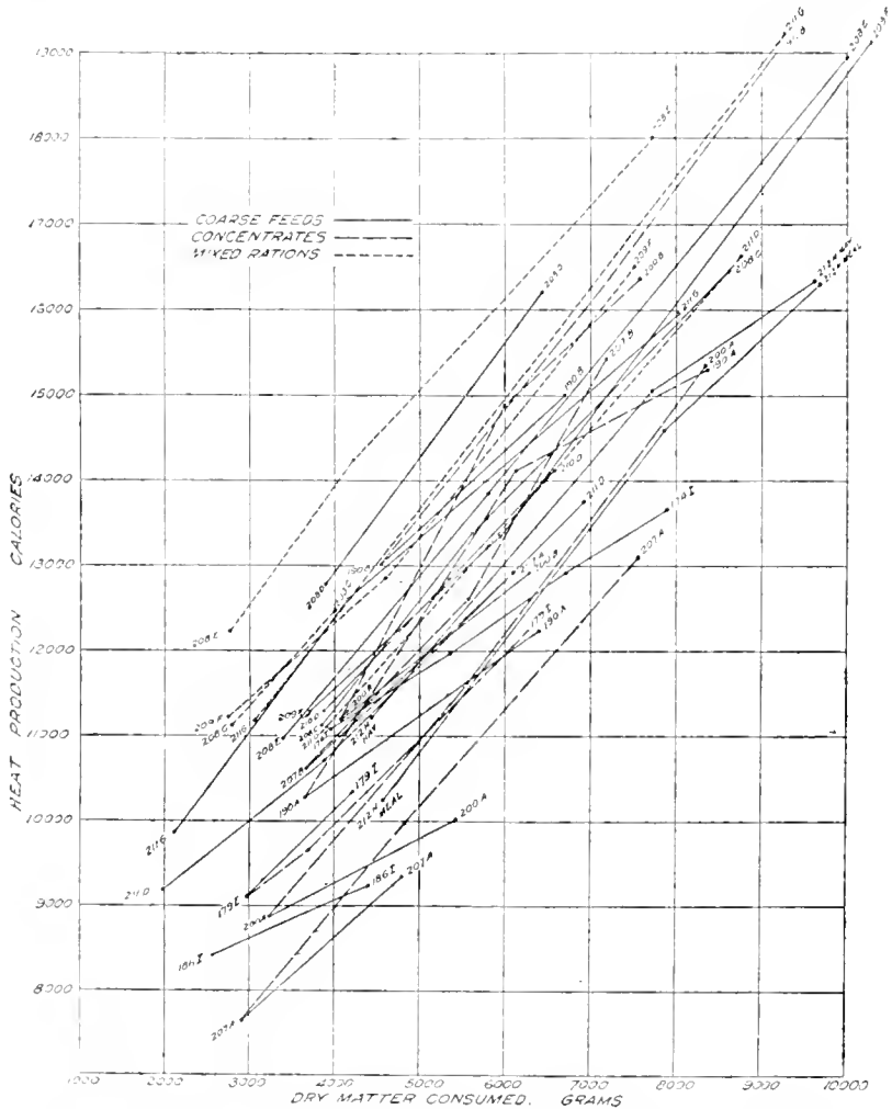
FIG. 2.—Graph showing the relation of heat production to dry matter consumed; computed per 500 kg. live weight.
