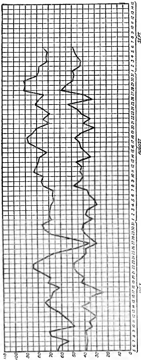
FIG. 4.—Curve showing the maximum and minimum temperature records in the Hudsonian zone (whitebark-pine association).
