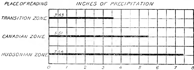
FIG. 2.—Diagram showing the total precipitation in the Transition, Canadian, and Hudsonian grazing zones during July, August, and September, 1909, inclusive.
