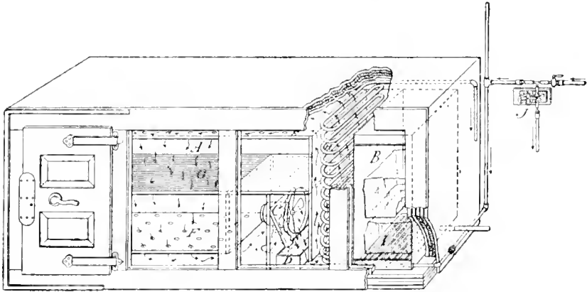
FIG. 1.—Constant-temperature humidior.
