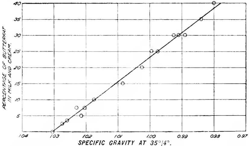
FIG. 2.—Specific gravity of milk and cream at 35°/4° C., showing relation between density and percentage of butter fat
