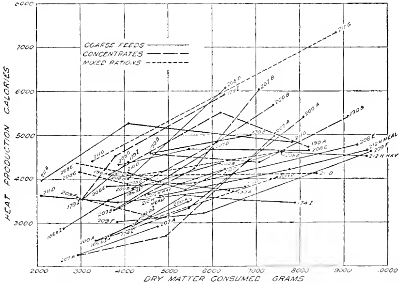
FIG. 1.—Graph showing the dry matter eaten and the increments of heat production due to standing; computed per 500 kg. live weight per 24 hours.
