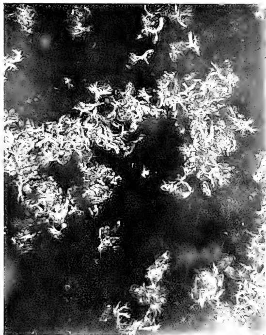
FIG. 3. The crystal form of the acetyl derivative of thyroxin.
