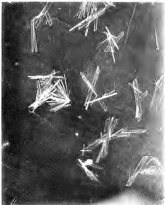
FIG. 9. The zinc salt of thyroxine which separates as long, flat blades in bundles and rosettes.
