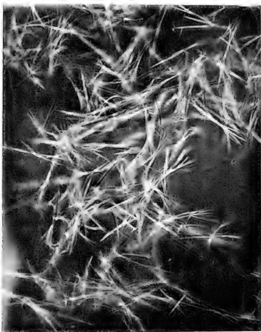
FIG. 16. Crystals of thyroxin in the amino carboxyl form.
