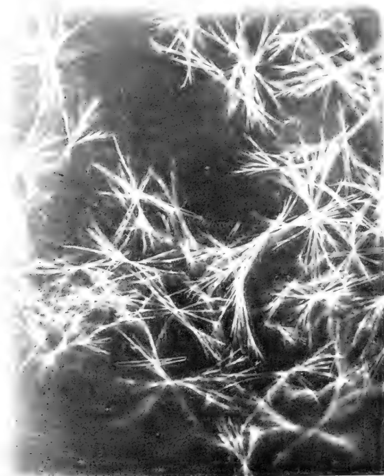
FIG. 22. The crystals of the amino hydrate form of thyroxin.
