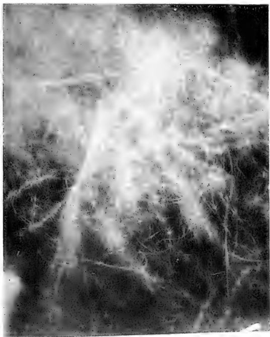
FIG. 19. A mixture of amino carboxyl crystals changing into the keto form of thyroxin. The long needles are crystals of the amino carboxyl form of thyroxin.
