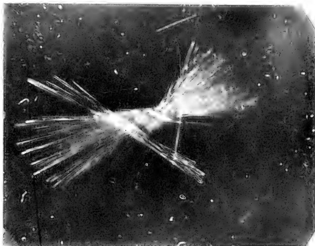
FIG. 2. The free form of thyroxin separated as a sheaf of needles.
