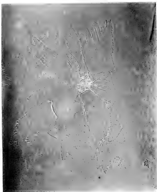
FIG. 13. The disodium salt of the acetyl derivative separated from a sodium acetate solution.
