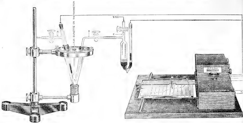
Bovie Hydrogen ion Outfit, with diagrammatic illustration of connections
