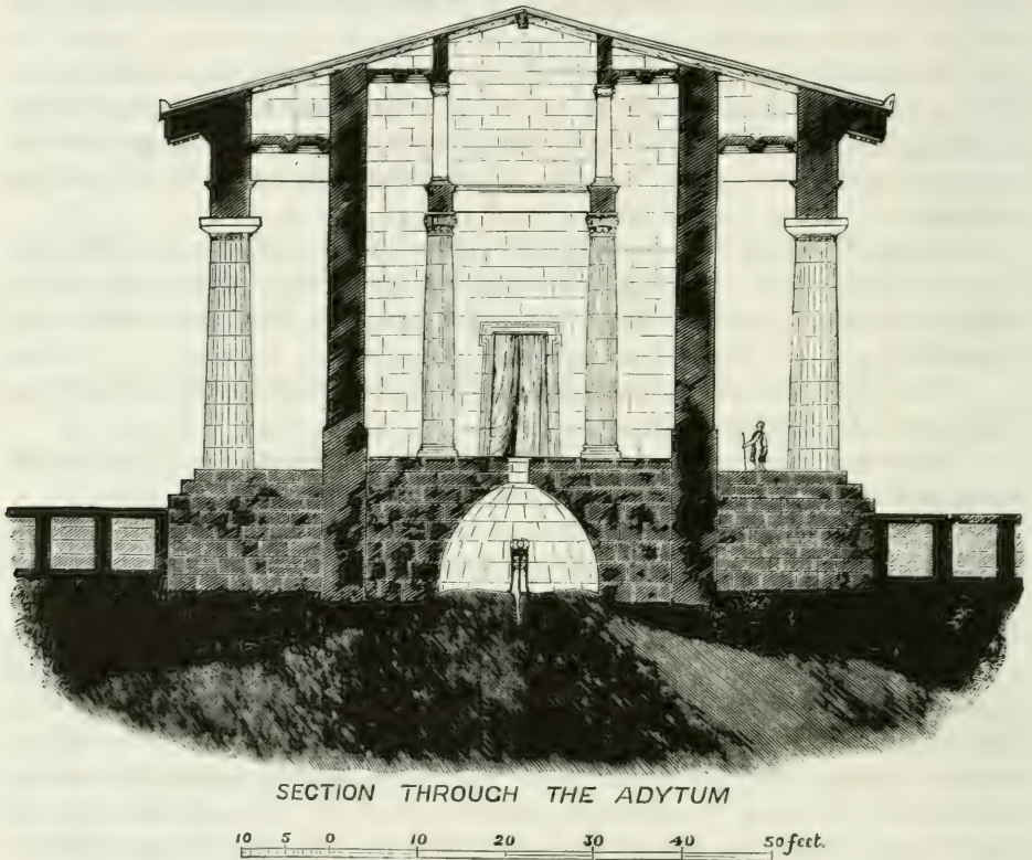
FIG. 13.—CONJECTURAL SECTION.
