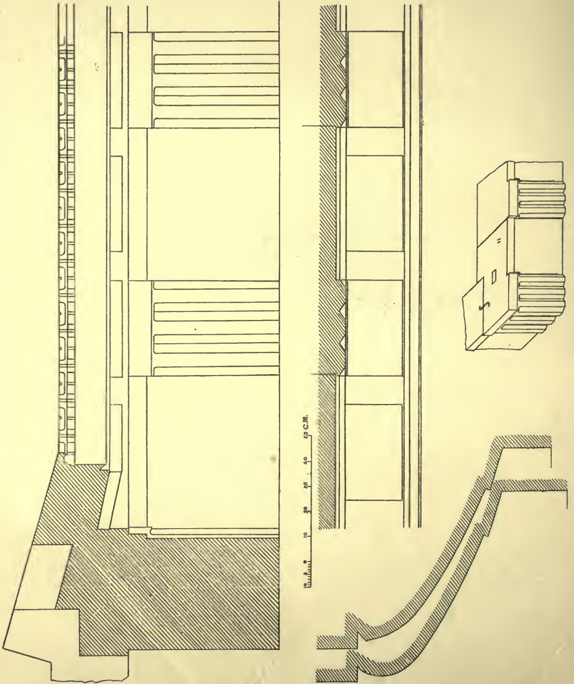
FIG. 11.—DETAILS OF THE SELINUNTINES' HOUSE (IX).
