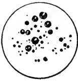
Fig. 1.—Spherical cavities in artificial ruby as seen at one time (enlarged 75 diameters).
