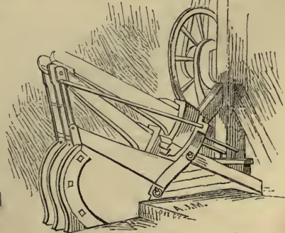
FULLING-STOCKS.
