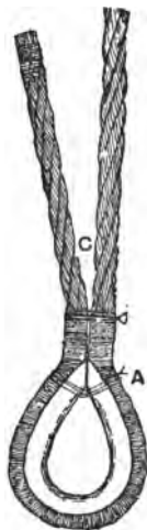
Fig. 181.—Wire Rope ready for Splicing.
