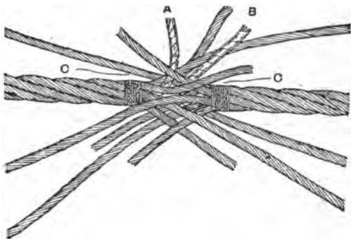
Fig. 178.—“Marrying” a Wire Rope Splice.
