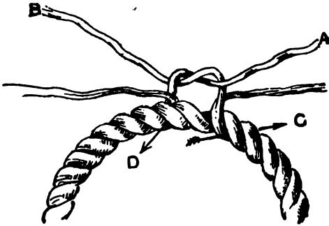
Fig. 121.—Finishing off Grommet.
