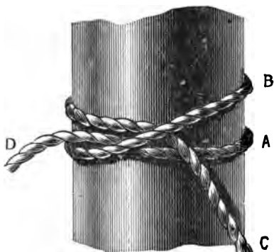
Fig. 97.—Beginning Turk's Head.
