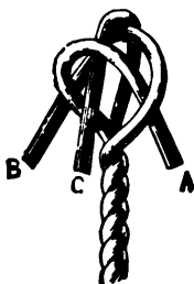
Fig. 86.—Crowning Complete.
