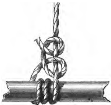
Fig. 30.—Rolling Hitch.
