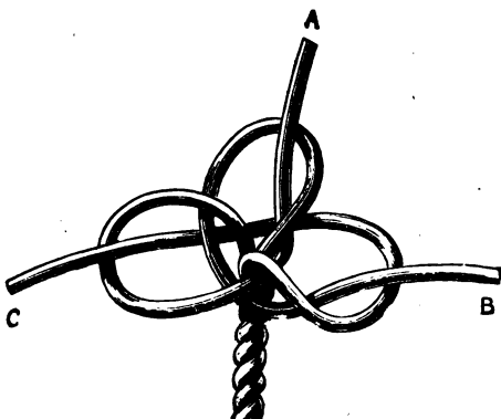
Fig. 93.—Diamond Knot before Hauling Taut.
