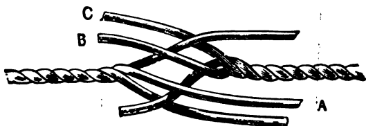
Fig. 113.—Beginning Short Splice.
