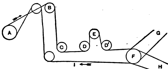
Fig. 177.—Colliery Band Rope Driving System.
