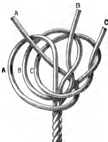
Fig. 90.—Beginning Matthew Walker Knot.
