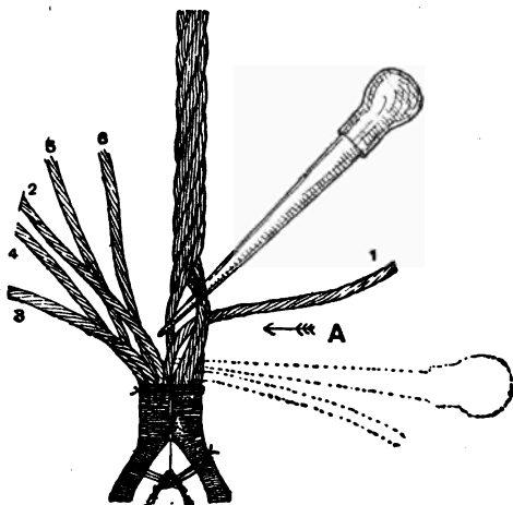
Fig. 182.—Right-handed Splice, First Tuck.
