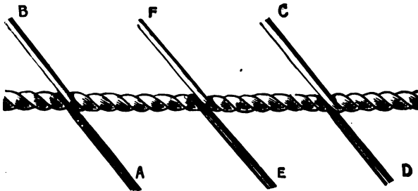
Fig. 116.—Long Rope Splice.
