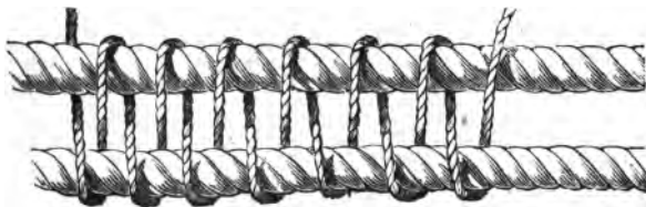
Fig. 78.—Nipping.
