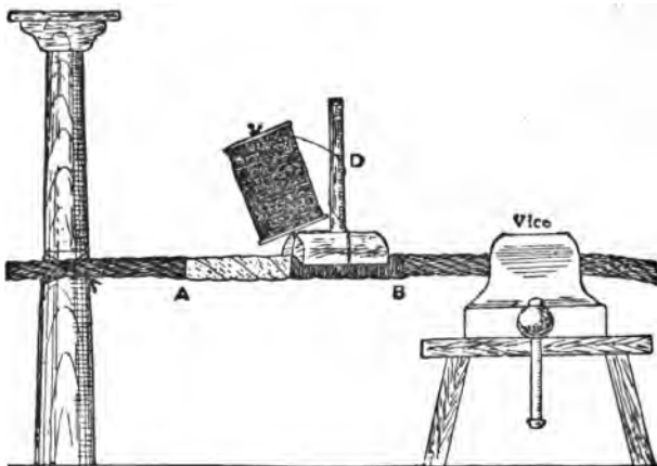
Fig. 179.—Method of Serving Wire Rope.
