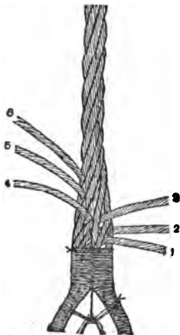
Fig. 183.—Right-handed Splice, all Ends Tucked Once.
