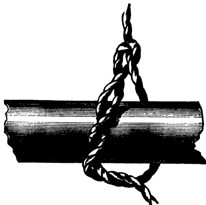
Fig. 26.—Timber Hitch.
