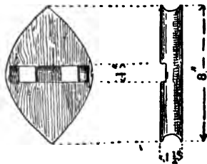
Fig. 157.—Side Piece of Pilot Ladder.
