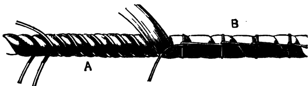
Fig. 126.—Worming, Parcelling, and Marling.
