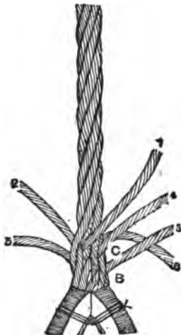
Fig. 185.—Left-handed Splice, all Ends Tucked Once.
