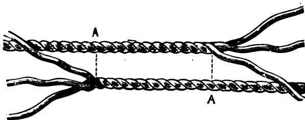
Fig. 118.—Beginning Cut Splice.
