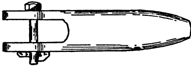
Fig. 200.—Plan of Solid Socket with Open End.
