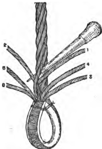
Fig. 184.—Left-handed Splice, First Tuck.
