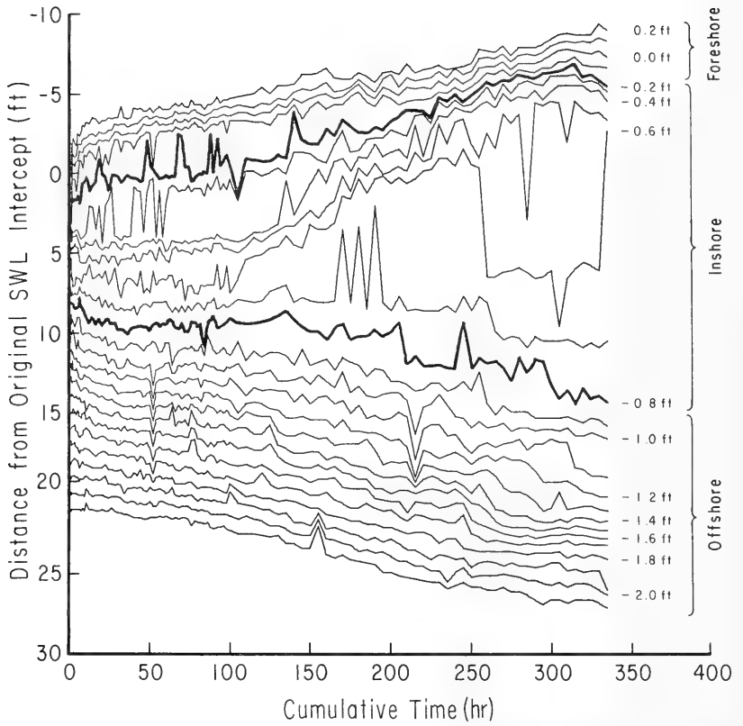
Figure 13. Profile changes along range 7, experiment 71Y-10.
