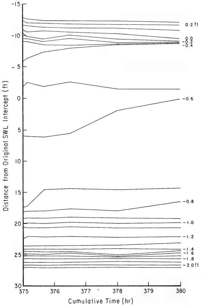
Figure 34. Profile changes along range 3 in experiment 71Y-06 between 375 and 380 hours.
