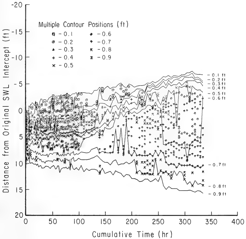
Figure 27. Changes in the inshore zone along range 7, experiment 71Y-10.
