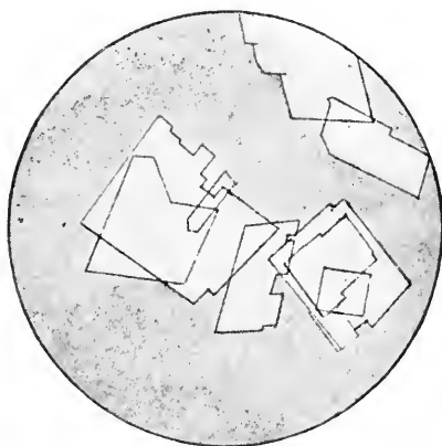
FIG. 6.—Cholesterin from Cystic Fluid.
