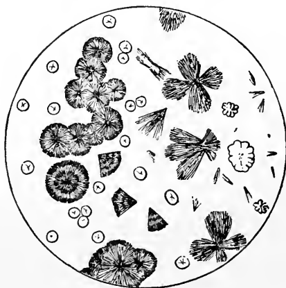
FIG. 9.—Creatinine Zinc Chloride from Urine.
