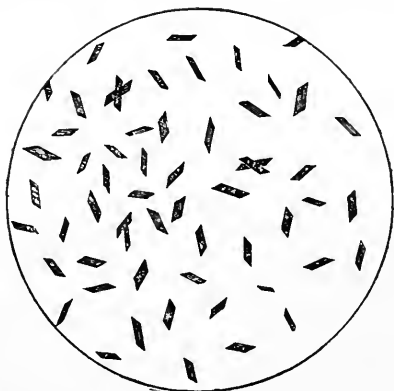
FIG. 4.—Hæmatin Hydrochloride, Hæmin Crystals.
