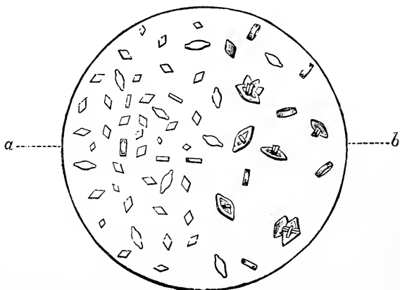
FIG. 8.—Uric Acid: (a) from alkali urate by the addition of hydrochloric acid; (b) spontaneously deposited from urine.
