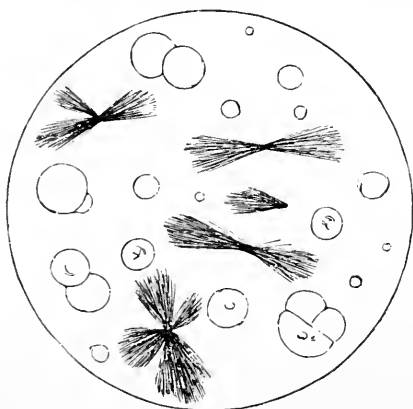
FIG. 5.—Leucine and Tyrosine.
