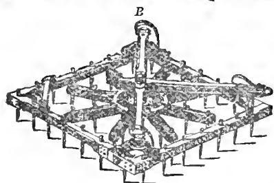
Patented April 13, 1880.
