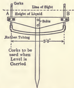
FIG. 98. Water or hose level (after Davidson).
