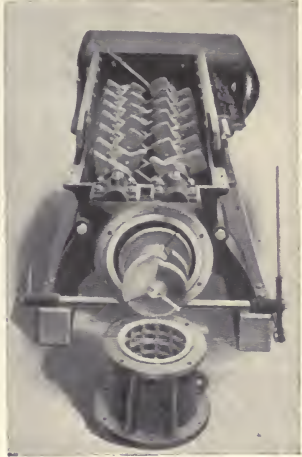
FIG. 16. Tile machine. This machine mixes the clay and forces it through a die onto the table shown in Fig. 17.
