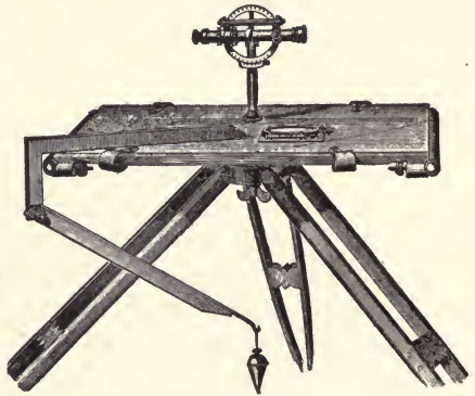
FIG. 103. A planetable.
