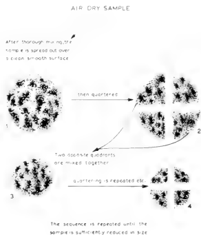
Fig. 8.6 A system of quartering for reduction in sample size.
