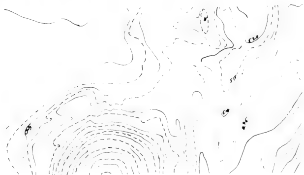
Fig. 5.4 Rough plan at 1:2500 scale with 5 ft contours.
