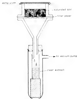
Fig. 8.8 Apparatus used for saturation moisture extraction and the determination of moisture equivalent.
