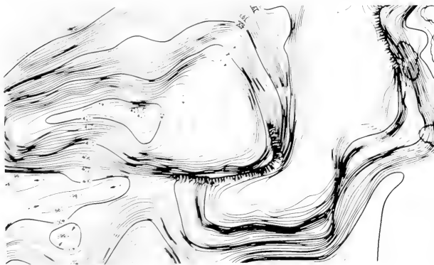
Fig. 5.1 1 ft contours at scale 1:500 are often difficult to read when abrupt changes in topography are to be delineated, and less detailed contour plans may give a clearer overall picture.
