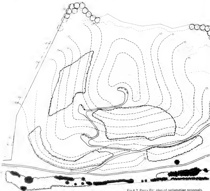
Fig 4.2 Percy Pit: plan of reclamation proposals.
