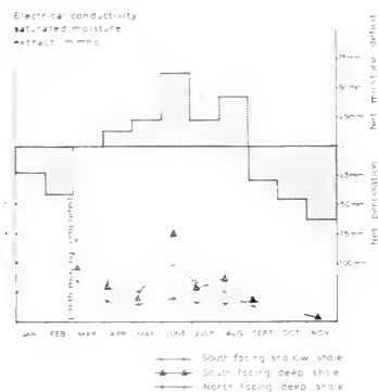
Fig. 8.4 Variation of salinity with water movement at Roddymoor, March - November 1968.
