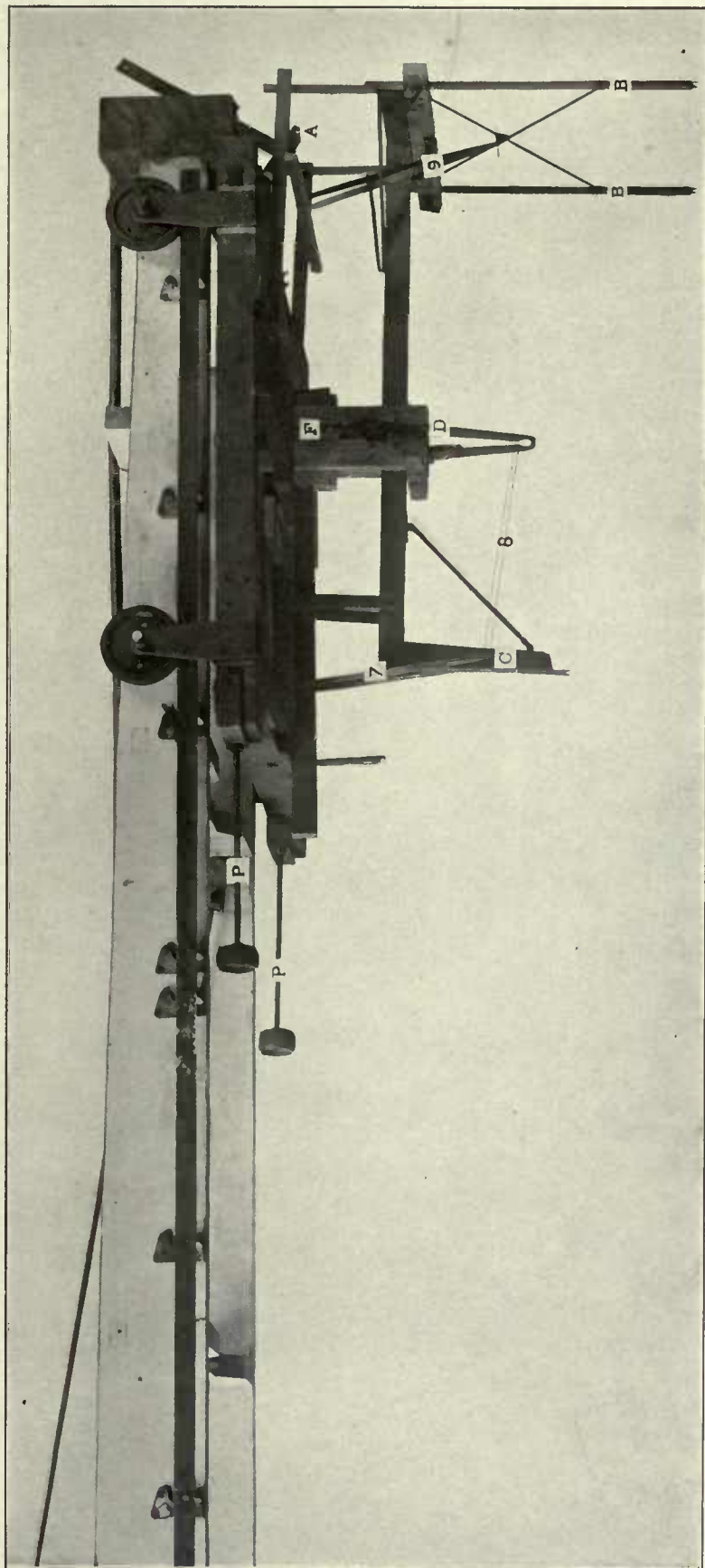
OVERHEAD LAUNCHING APPARATUS
