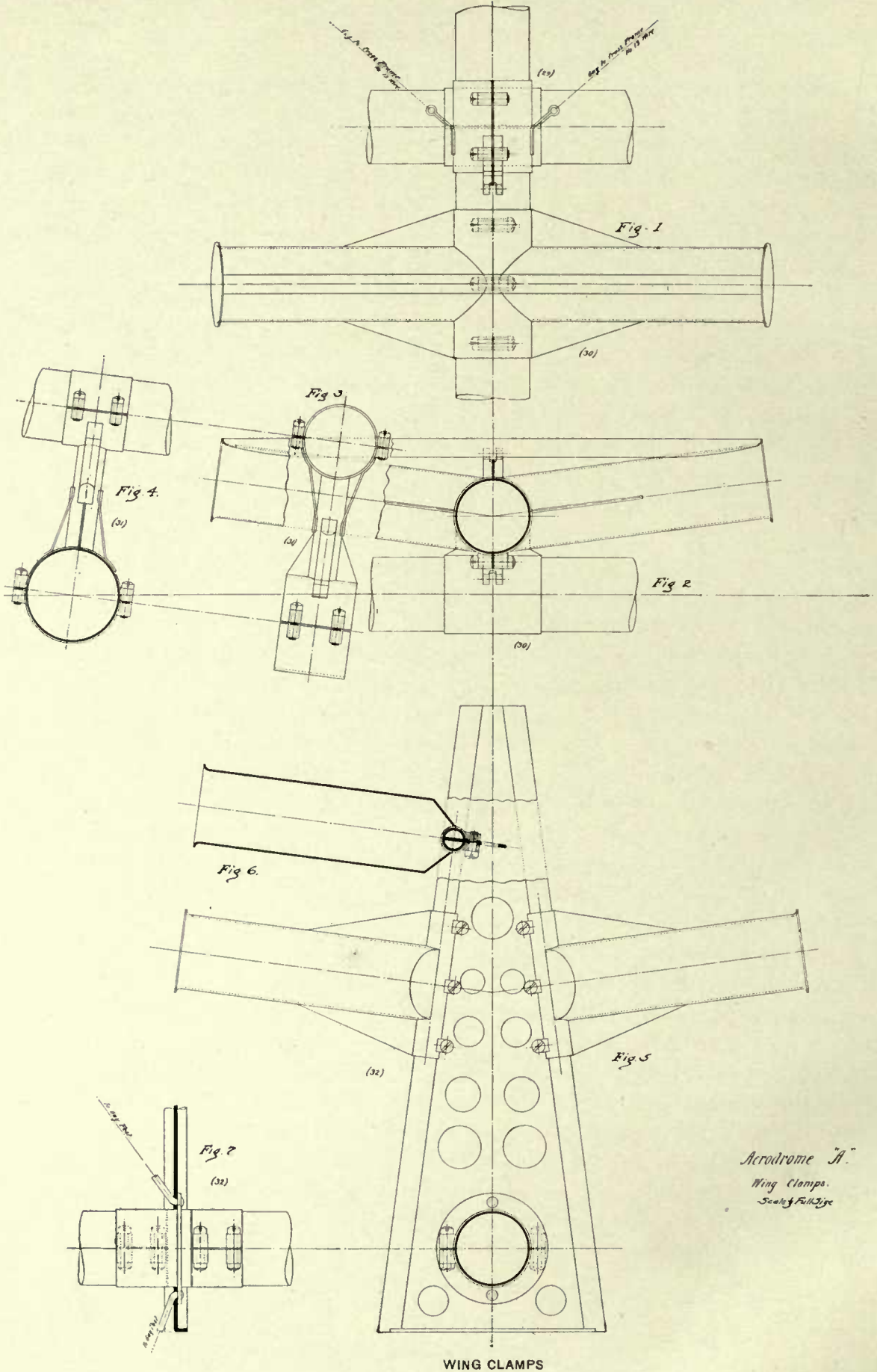
WING CLAMPS
