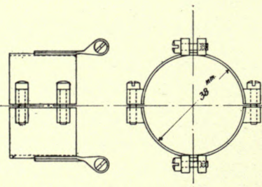
Fig. 11. Fitting at 'dd'
