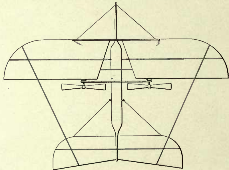
EARLY TYPES OF WINGS AND SYSTEMS OF GUYING
