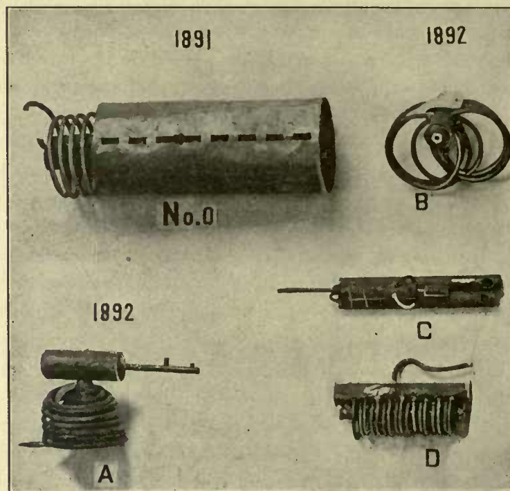
FIG. 3. Boilers in use in 1891-1892.
