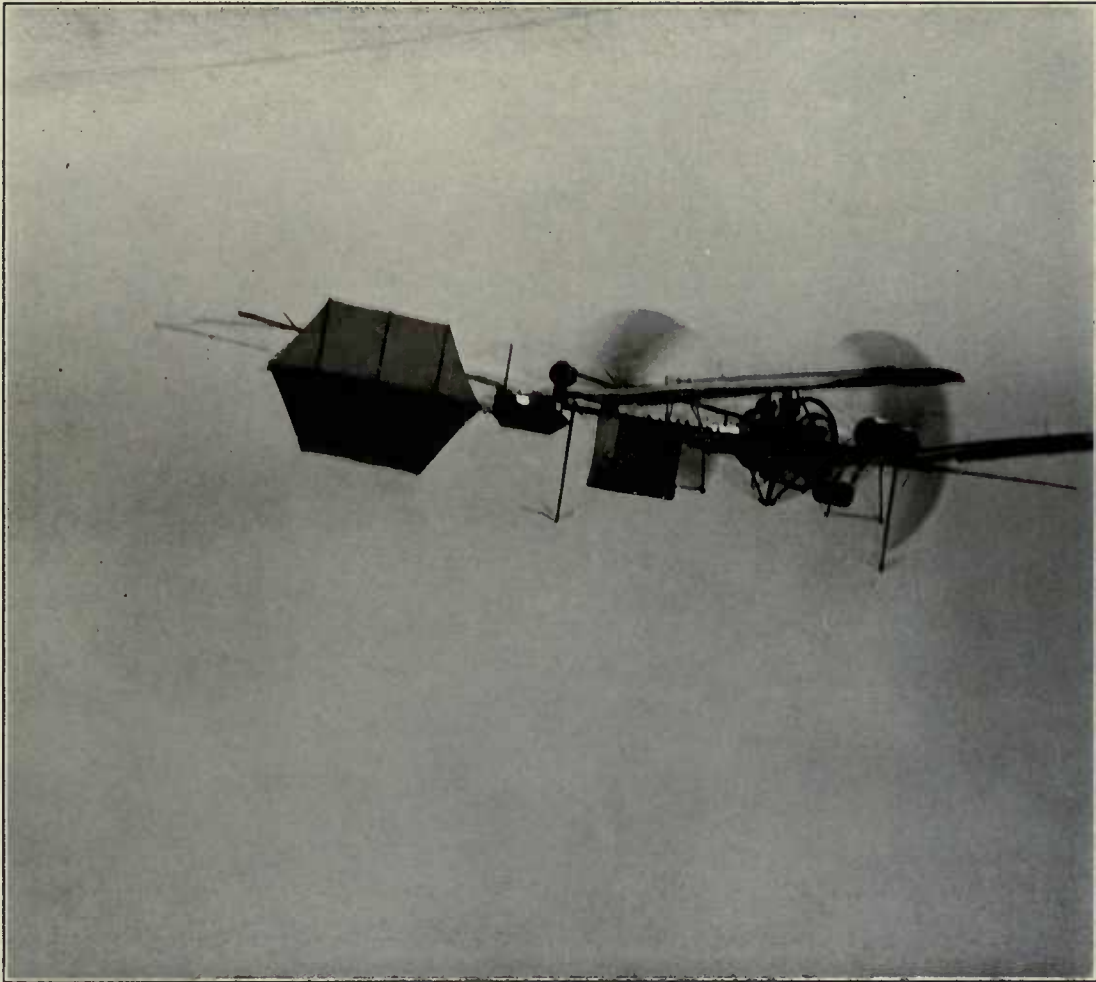
QUARTER-SIZE MODEL AERODROME IN FLIGHT, AUGUST 8, 1903
