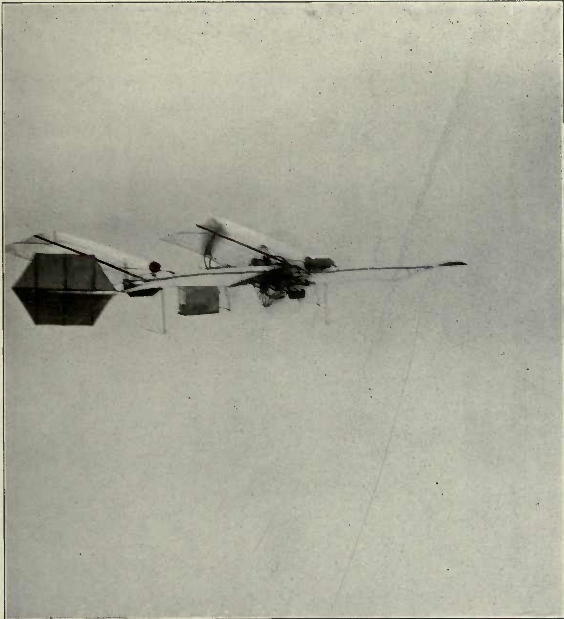
QUARTER-SIZE MODEL AERODROME IN FLIGHT, AUGUST 8, 1903
