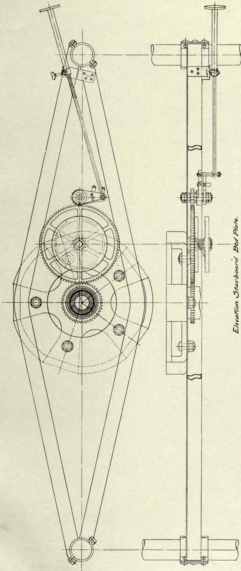
ENGINE OF AERODROME A. ELEVATION STARBOARD BED PLATE, SPARKING MECHANISM
