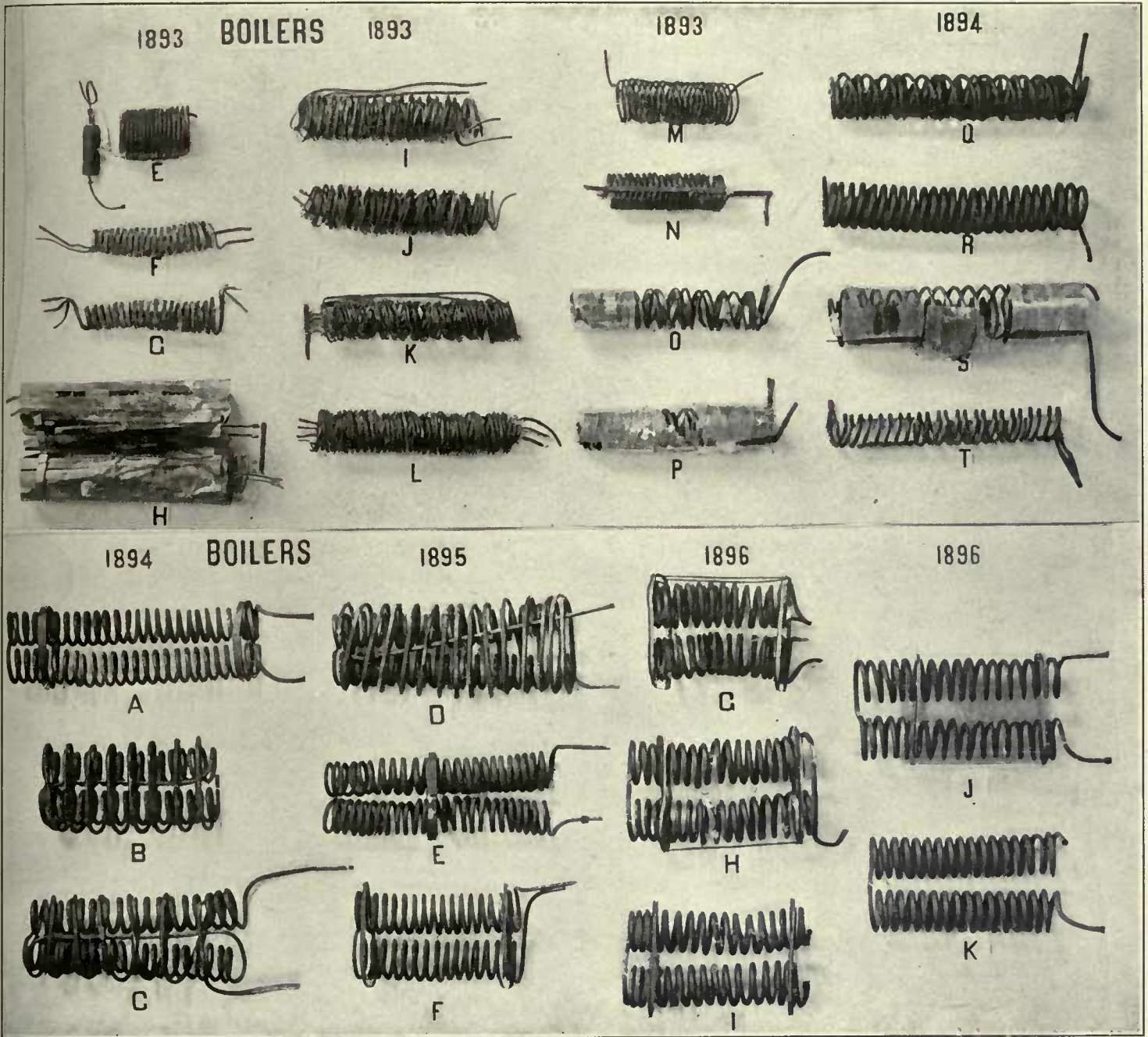
BOILERS OF AERODROMES
