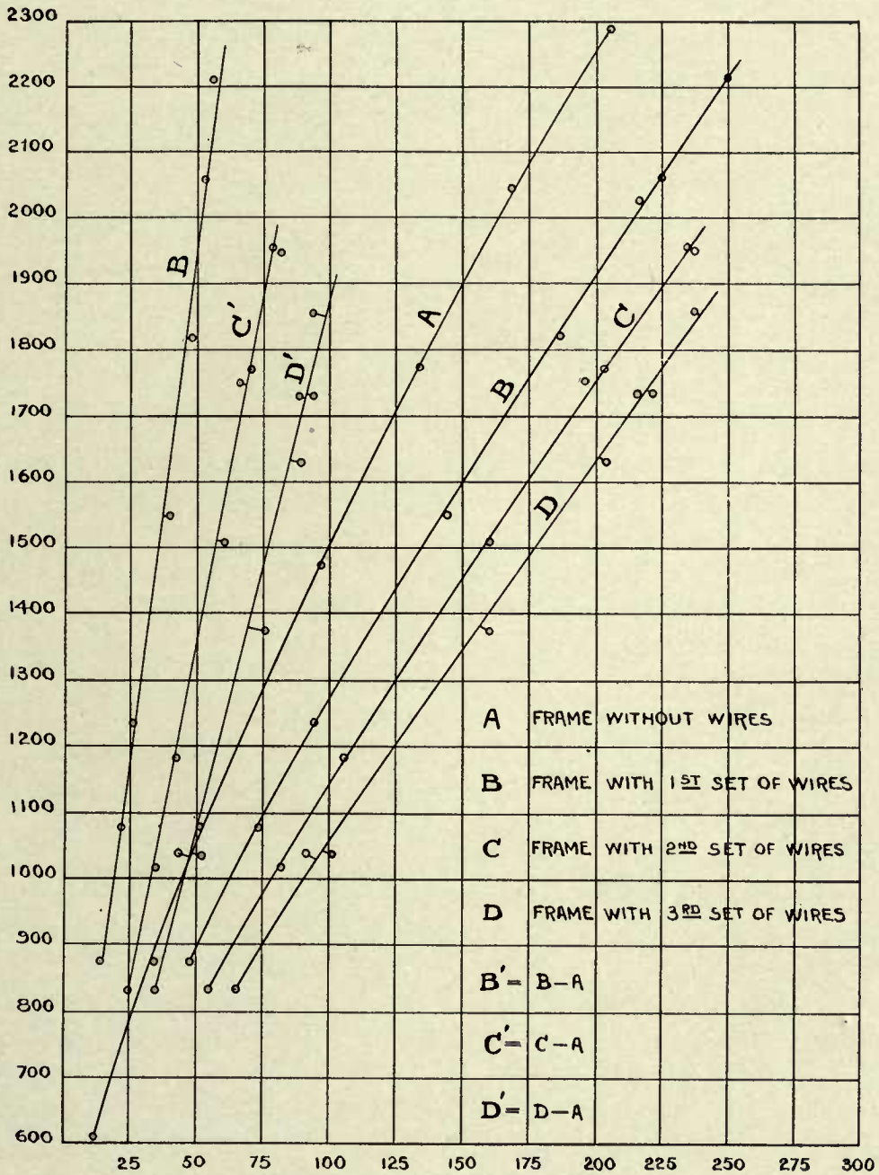
RESISTANCE OF WIRES AT GIVEN VELOCITIES ORDINATES=VELOCITY IN FEET PER SECOND ABSCISSAE = RESISTANCE IN GRAMMES
