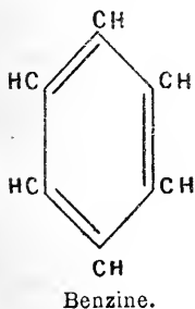
Benzine.
