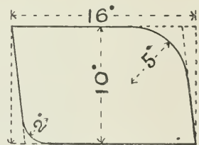
DETAIL OF SEAT-ENDS
