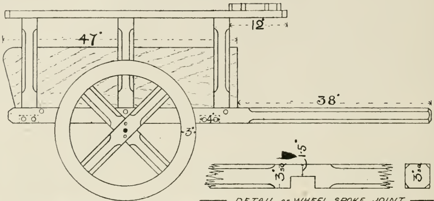
SIDE ELEVATION
