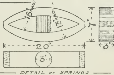
DETAIL OF SPRINGS
