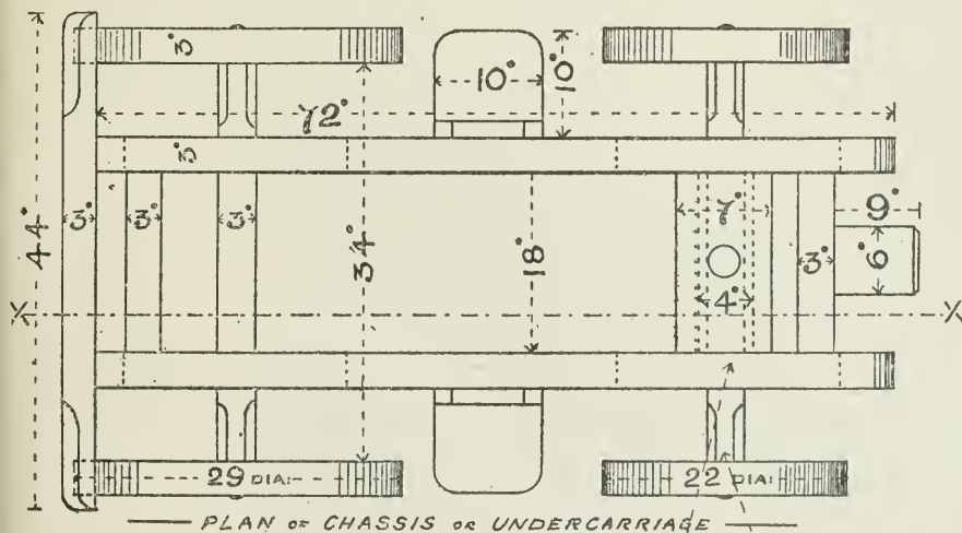
PLAN OF CHASSIS OR UNDERCARRIAGE
