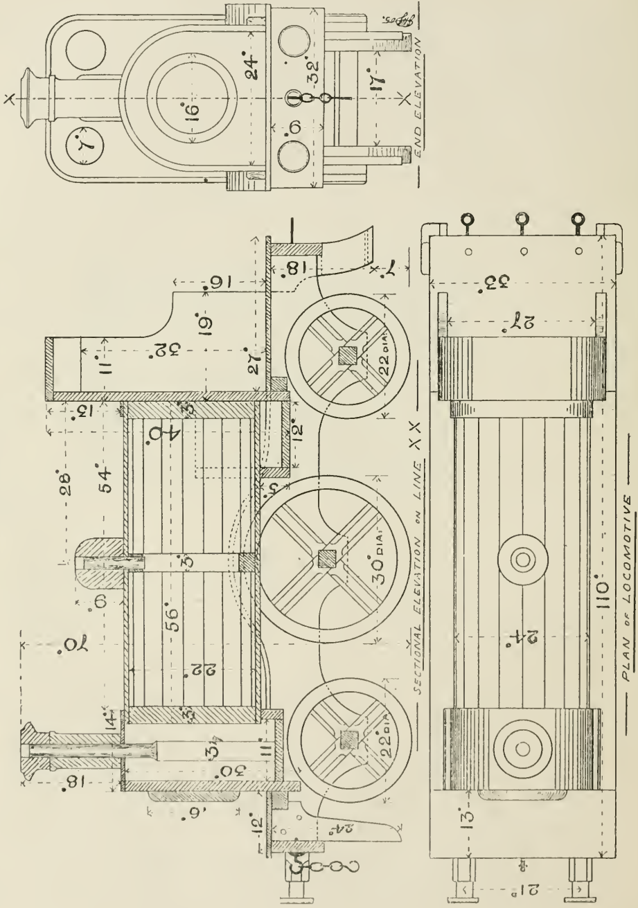
SECTIONAL ELEVATION OF LOCOMOTIVE. PLAN AND END VIEW.
