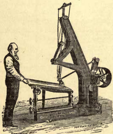
PEBBLING JACK.
