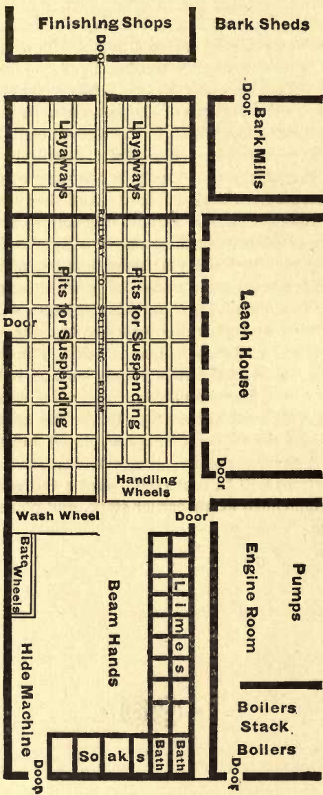
GROUND PLAN OF TANNERY.
