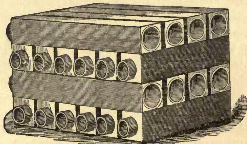
PLAIN SQUARE LIQUOR PIPES.
