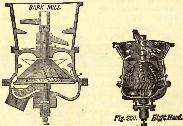
BARK MILLS.
