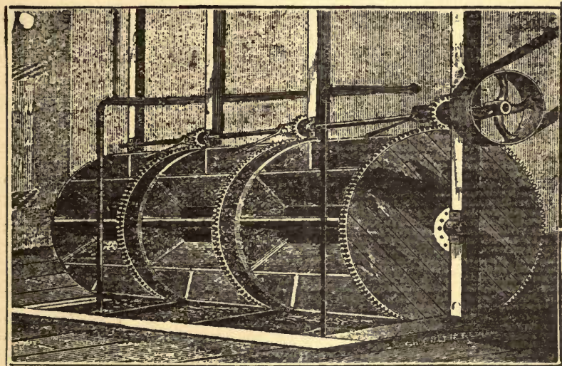
BATE WHEELS.
