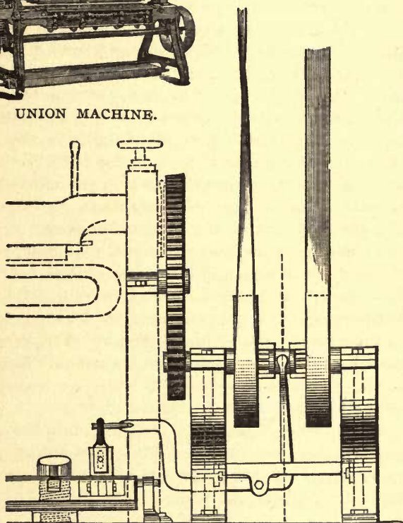
FRICTION GEAR FOR UNION MACHINE.
