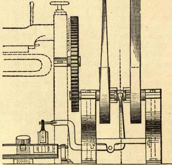
FRICTION GEAR FOR UNION MACHINE.
