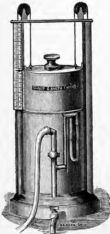
FIG. 8.—Hutchinson's Spirometer.
