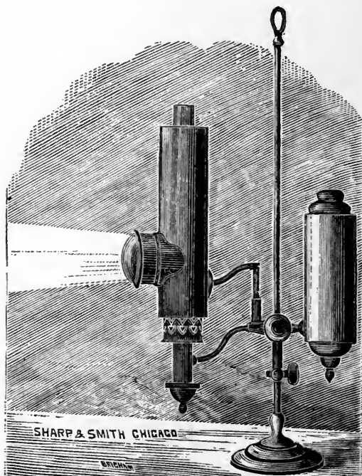
FIG. 51.—Modification of Mackenzie's illuminator which may be used either with a student's lamp or an Argand gas burner.
