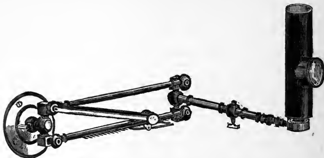
FIG. 50.—Mackenzie's rack-movement bull's-eye condenser.
