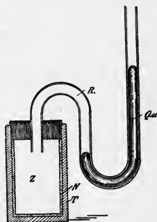
Fig. 3. PFEFFER'S osmotic cell. T , porous pot; N , precipitation membrane; R , manometer containing mercury, Qu ; Z , sugar solution.
