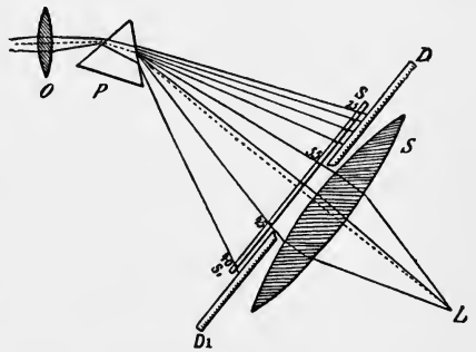
Fig. 26. Diagrammatic sketch of a spectrophore (after REINKE, Bot. Ztg., 1884, pl. I, fig. 2). O , projection lens; P , prism; SS , scale of \lambda = 40 to \lambda = 75 ; D , D 1 , diaphragm for cutting off extraneous rays; S , converging lens; L , position of the plant experimented on.
