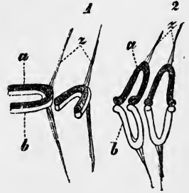
Fig. 57. Diagram to illustrate the separation of the chromosomes. z , spindle threads; a and b , the two longitudinal halves of the chromosome. (From the Bonn Textbook.)
