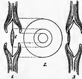
Fig. 18. 1. Bordered pit of Pinus sylvestris in tangential section; 1, the torus. 2. Surface view of the pit; corresponding regions are united by dotted lines. 3. As in 1, but the torus is pressed against the pit on the left. (After Russow, diagrammatic.)
