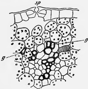
Fig. 13. Water stoma of Vicia faba in section. sp , the stoma; g , vessels abutting on the intercellular spaces. (After HABERLANDT, 1895, pl. 3.)
