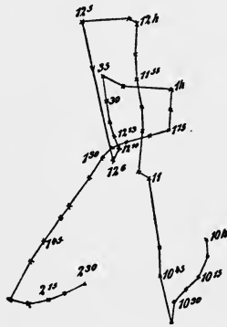
Fig. 162. Projection curve of Phycomyces nitens , after FRITZSCHE (1899). x 200.
