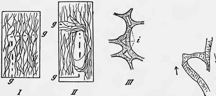
Fig. 100. Mode of growth of transplanted portion of beet. I , tangential section through the upper end of a portion of tissue inserted in the normal orientation. The limits of the tissue are indicated by the dotted lines gg . The longitudinal lines indicate vessels. II , a similar section of an inverted graft. The vascular bundles are developing almost entirely in the long axis; I and II about natural size. III , individual cells from the area of fusion; i , intercellular spaces and thickened cell-walls. \times about 350. After VÖCHTING, 1892.
