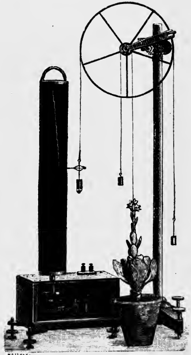
Fig. 84. PFEFFER'S auxanometer, as manufactured by ALBRECHT of Tübingen.
