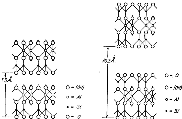
TEXTFIGURE 4. — Above : Two building units of crystalline structure of soil colloids. — Below : Showing proposed crystalline structures of two general types of soil colloids, kaolinite and montmorillonite. (From KELLEY, JENNY and BROWN, 1936).
