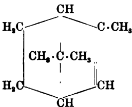
Fenchylalkohol
