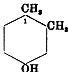
Dimethyl-1.2-oxy- 4-benzen
