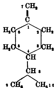
\Delta^{1(7)} -p-Menthan
