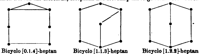
Bicyclo [0.1.4]-heptan
