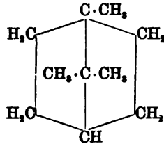
1.7.7-Trimethylnorcamphan, Camphan
