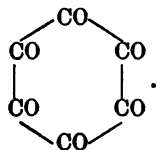
Trichinoyl
