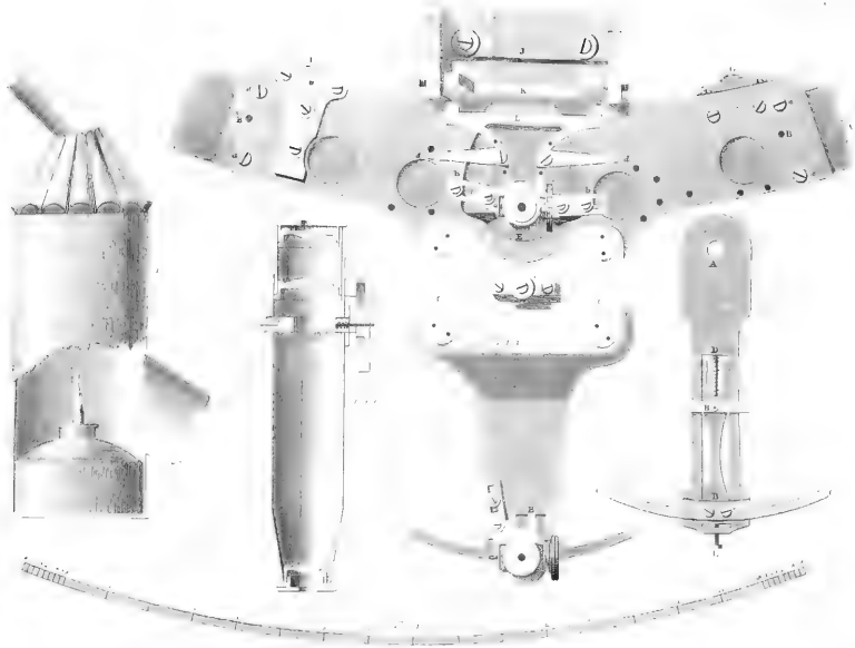
W. Thompson's Self-Propelling Apparatus
