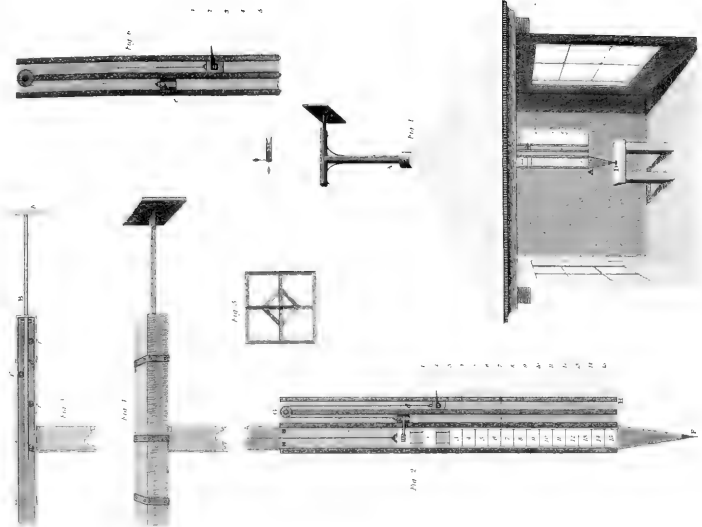
Reinhold's Anemometer
