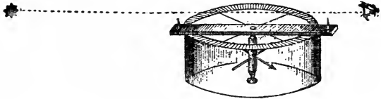
FIG. 3.—PIVOTED COMPASS
