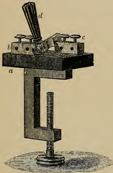
FIG. 17.—Key for opening or closing current.
