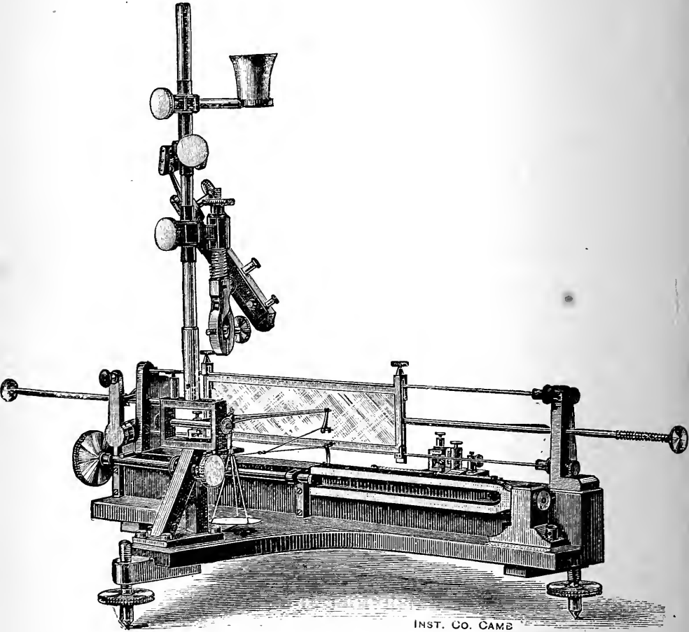
FIG. 55.—The spring myograph of du Bois Reymond.
