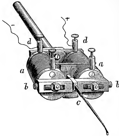
FIG. 27.—Electric chronograph. For description see text.
