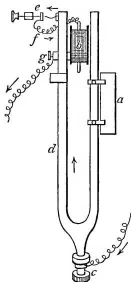
FIG. 39.—Tuning-fork arranged for causing a smoked-glass plate, a , to vibrate. b , electro-magnet; current passes in at c , along limb of fork, d , along platinum wire to platinum contact at e , thence by wire, f , to electro-magnet, b , thence back to battery by wire from g . When b is magnetised the limbs of the fork are drawn together and contact is broken at e . The limbs then fly back and again make contact at e , and so on.
