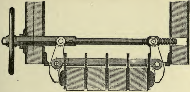
1. Section Showing the Friction-gear Applied to the Princeton, 1842, and to the Gun-carriages of the United States Iron-clad Fleet, 1862-67.
