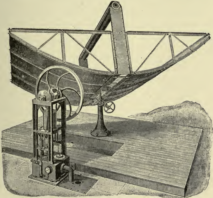
Ericsson's Sun Motor, Erected at New York, 1883.
