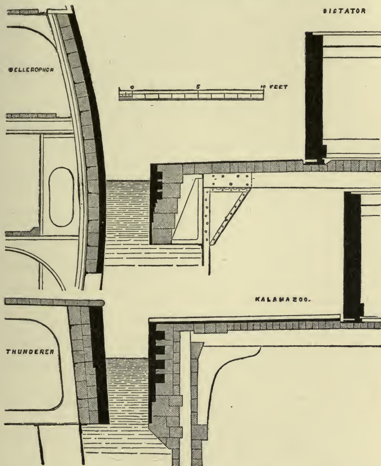
British and American Turreted Vessels Contrasted.
