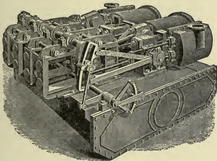
Motive Engine of the Destroyer.
