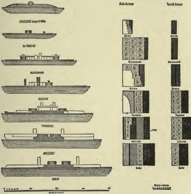
Development of the Monitor Idea.
