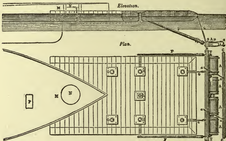
Obstruction Remover of Captain Ericsson.
