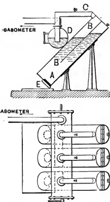
FIG. 36. Lequeux Generator.
