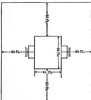
FIG. 4.—Space needed for 65 x 80 foot school-house if lighted on all sides and entirely shut in by buildings 40 feet high. Shows need of another type of building. An H-shaped building (See Fig. 7) would occupy two-thirds of the lot.
