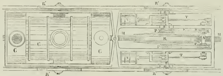
(Fig. 2. — Plan de la locomotive.)
