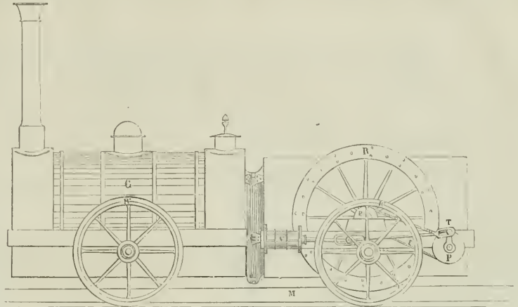
(Fig. 1. — Elevation de la locomotive.)
