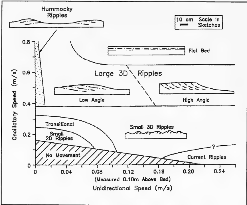
Figure 15. Stability fields for bed forms produced in very fine sand in collinear combined-flow water tunnel. Velocities were measured at 0.10 m above the bed. Note that "2D" considers a two-dimensional (straight-crested, which is usually representative of low energy conditions) bed form, while "3D" considers a three-dimensional (sinuous-crested, usually representative of high energy conditions) bed form (from Arnott and Southard (1990))
