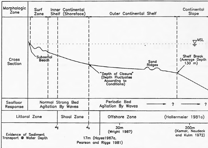
Figure 1. Continental shelf cross-sectional profile (site specific to the mid-Atlantic Bight of the United States). D_s and d_s (from Hallermeier (1981a)) refer to the seaward limit of surf-related effects, and the seaward limit to sand motion by normal waves, respectively
