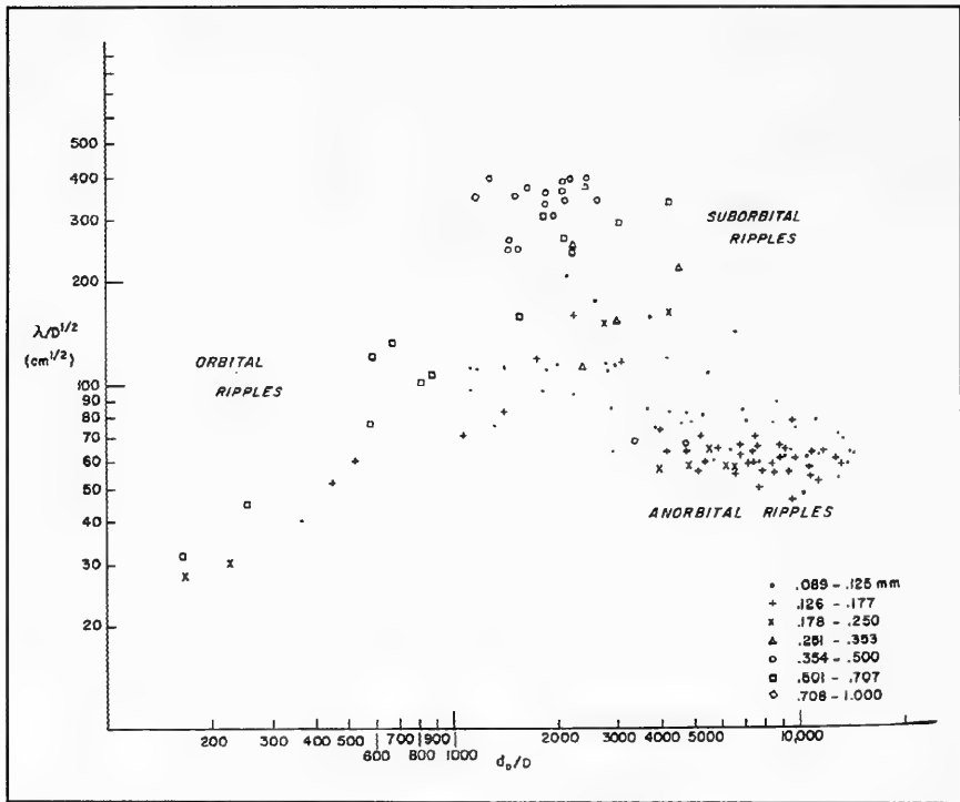
Figure 14. Classification of symmetric and reversing ripples based on the ratio of ripple length to square root of grain diameter ( \lambda/D^{1/2} ) and ratio of orbital diameter to grain diameter ( d_o/D ) (after Clifton (1976)) based on data from Inman (1957) and Dingler (1974)
