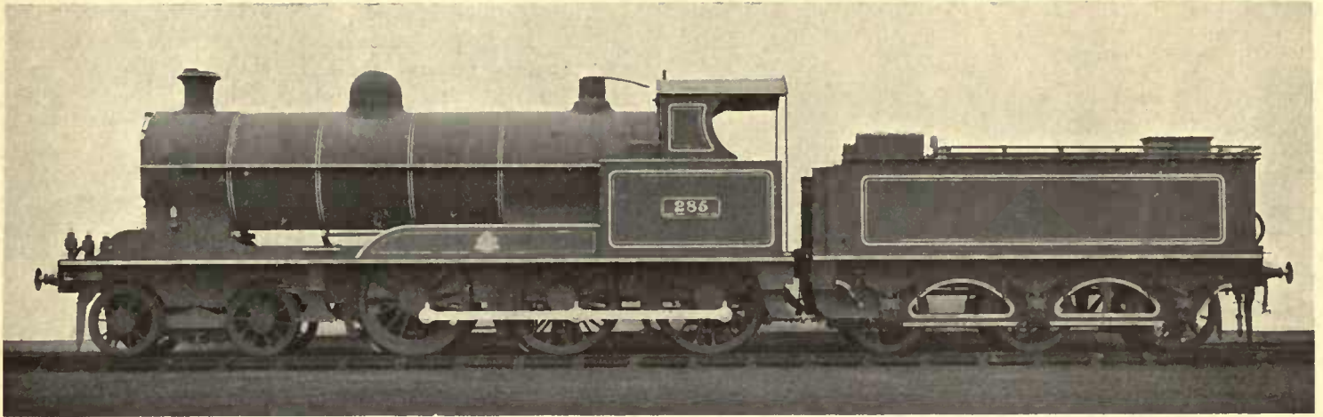
4—6—0 TYPE FAST GOODS LOCOMOTIVE, LONDON AND NORTH-WESTERN RAILWAY. MR. GEORGE WHALE, M.Inst.C.E., Chief Mechanical Engineer , CREWE.
