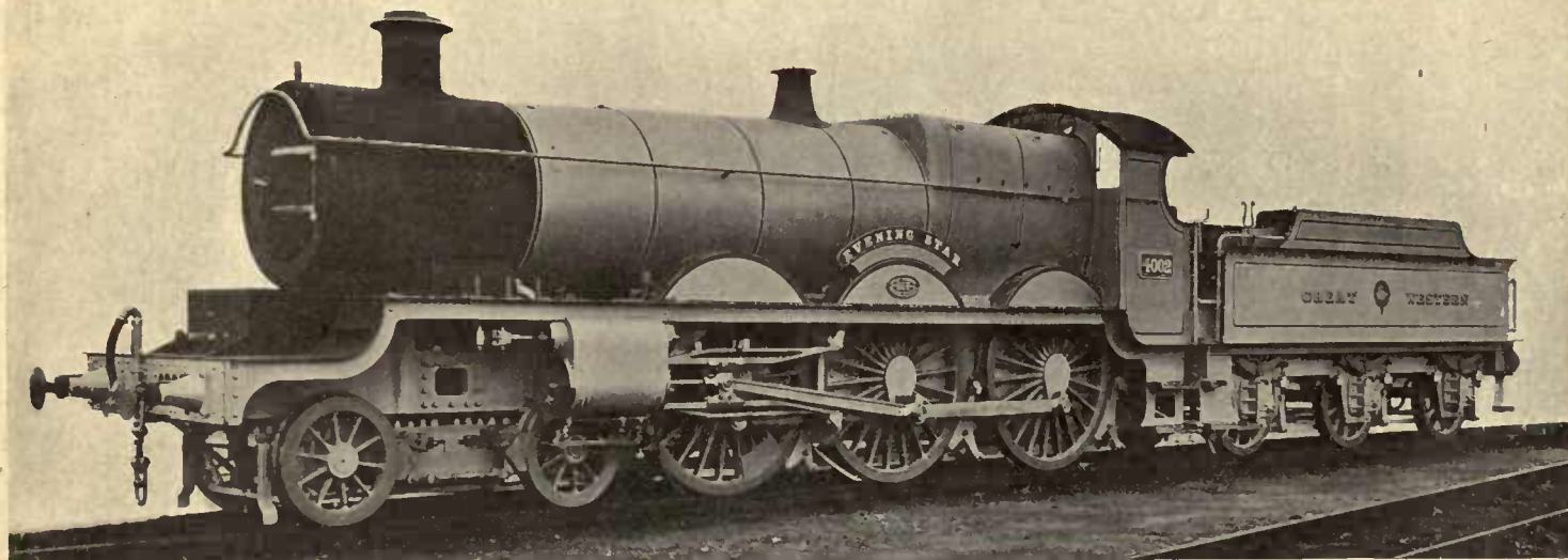
FOUR-CYLINDER SIMPLE (4—6—0 TYPE) EXPRESS LOCOMOTIVE, GREAT WESTERN RAILWAY. MR. G. J. CHURCHWARD, M.Inst.C.E., Locomotive Superintendent , SWINDON.
