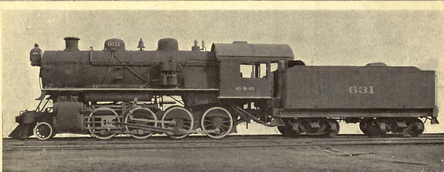
"CONSOLIDATION" (2-8-0 TYPE) FREIGHT LOCOMOTIVE, CHESAPEAKE AND OHIO RAILROAD, U.S.A. BUILT AT THE BROOKS WORKS OF THE AMERICAN LOCOMOTIVE COMPANY.
