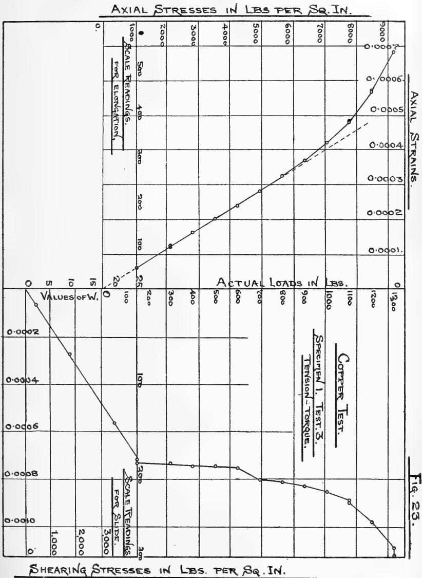
Fig. 23.—Copper Test by Tension and Torque.
