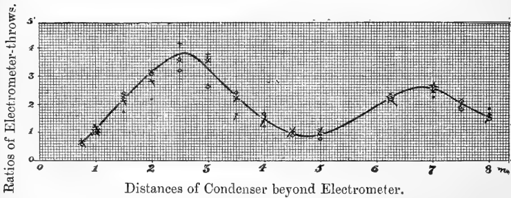
Fig. 8.—Experimental Results. Interference System for Medium Condenser. The several sets of readings are respectively indicated by *, o, †, and x.
