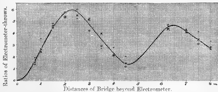
Fig. 7.—Experimental Results:—Interference System for Bridge of Negligible Resistance. Three sets of readings indicated by \cdot , \circ , and \times respectively.
