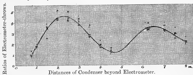
Fig. 7.—Experimental Results:—Interference System for Bridge of Negligible Resistance. Three sets of readings indicated by \cdot , \circ , and \times respectively.
