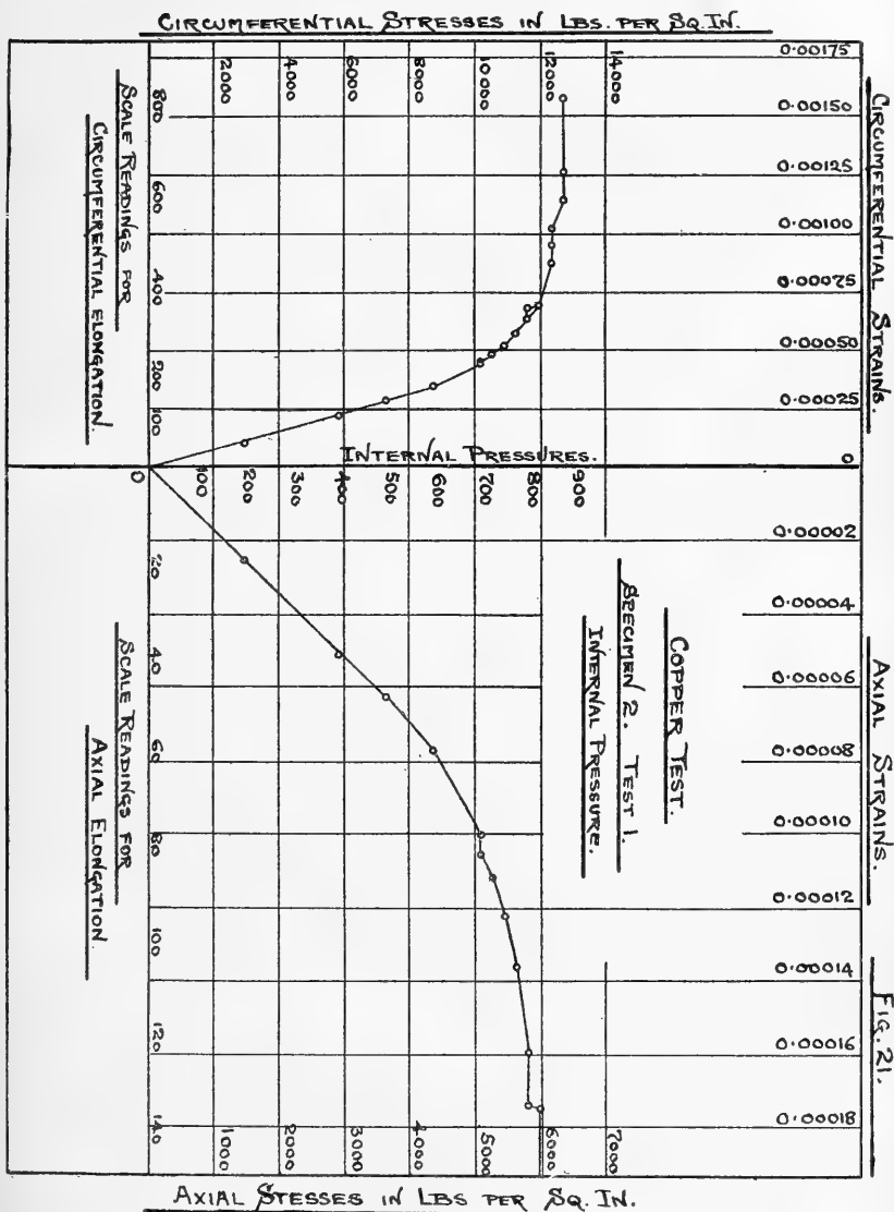
Fig. 21.—Copper Test by Internal Pressure.
