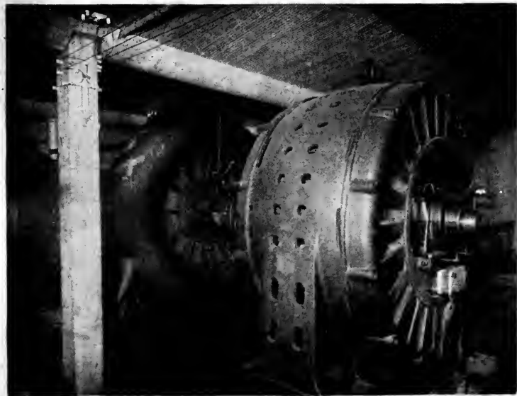
MAIN ARCH, WESTINGHOUSE EXHIBIT. 2,000 H. P. WESTINGHOUSE INDUCTION MOTOR.
