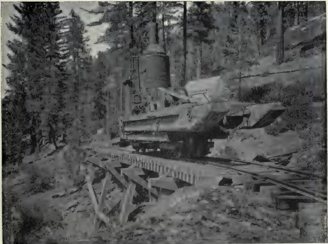
(2). Transporting skidder by rail on 3-foot track.—Lamoine, California.
