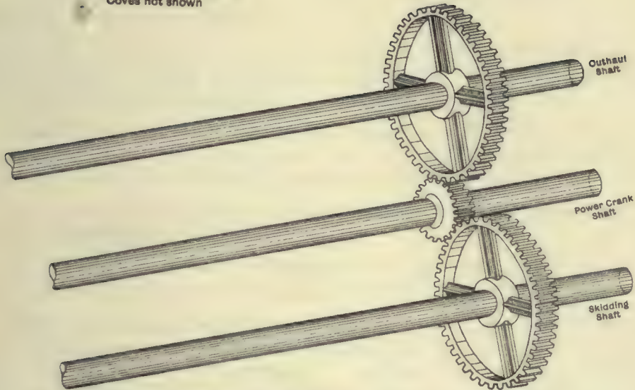
(1).—Gearing of Drum Shafts—Ordinary type of Skidder.
