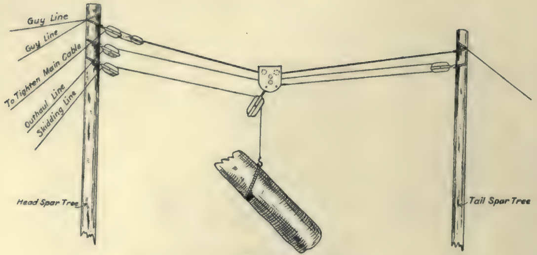
(1).—Overhead Skidding—ordinary type.
