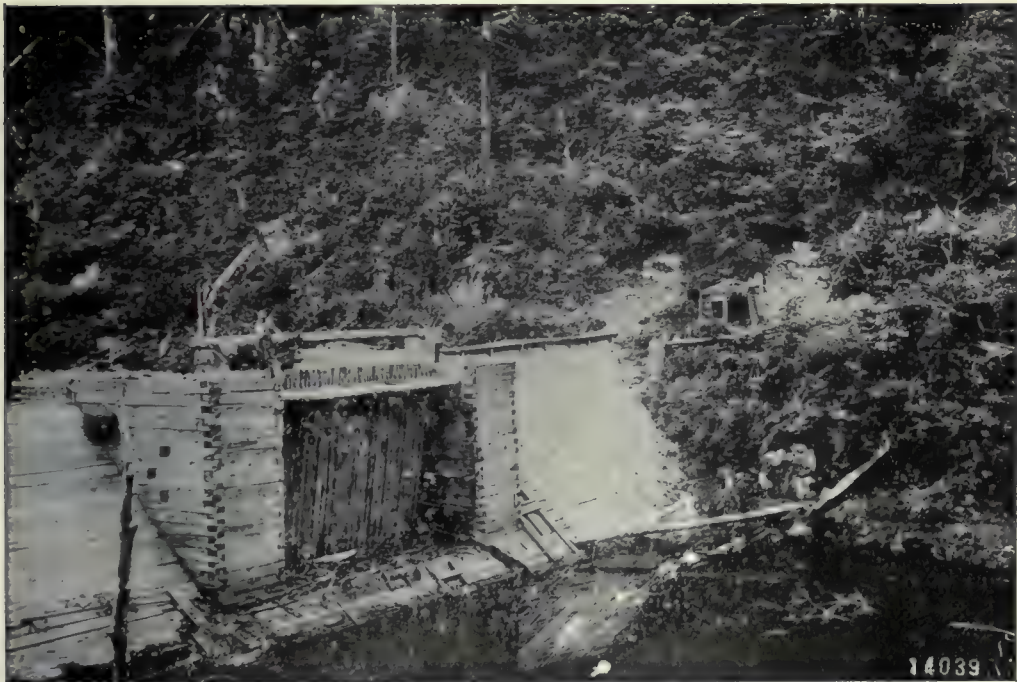
(2). Splash Dam raising water level 35 feet.—Blount County, Tenn. U. S. Forest Service Photo.
