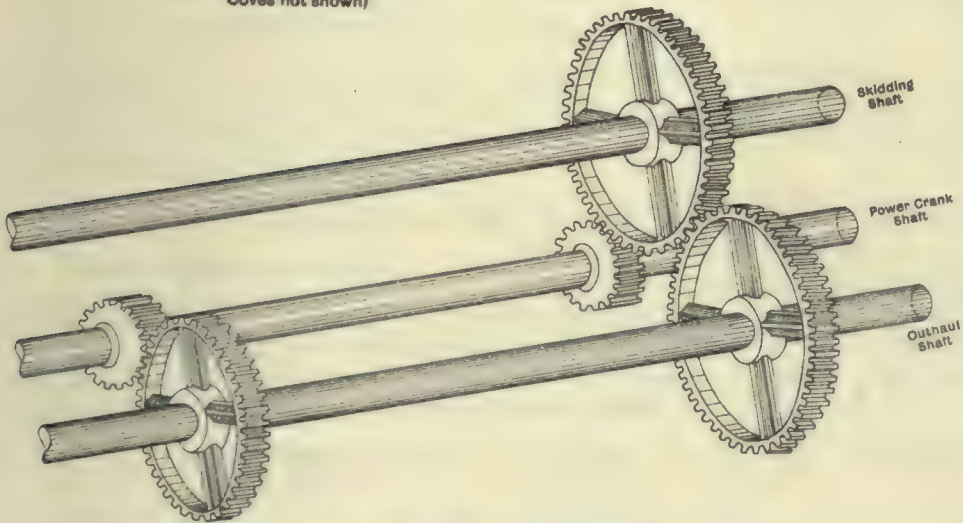
(2).—Gearing of Drum Shafts—Lidgerwood Interlocking Drum type.
