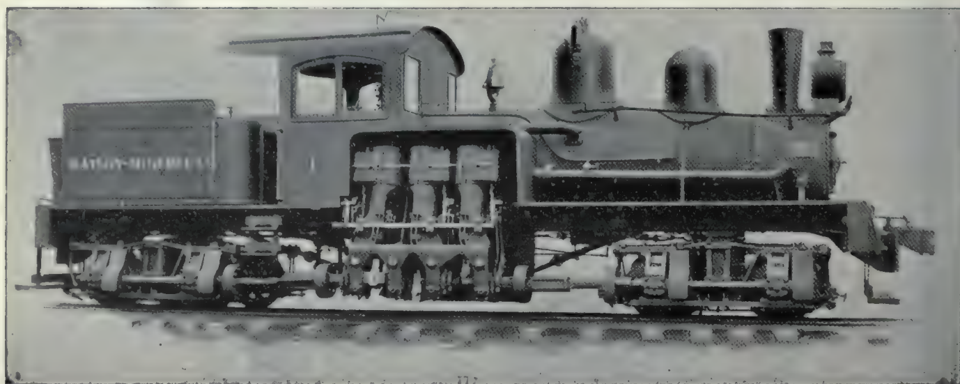
(2). 70 ton Shay geared Locomotive. (Built by the Lima Loco. and Machine Co.)
