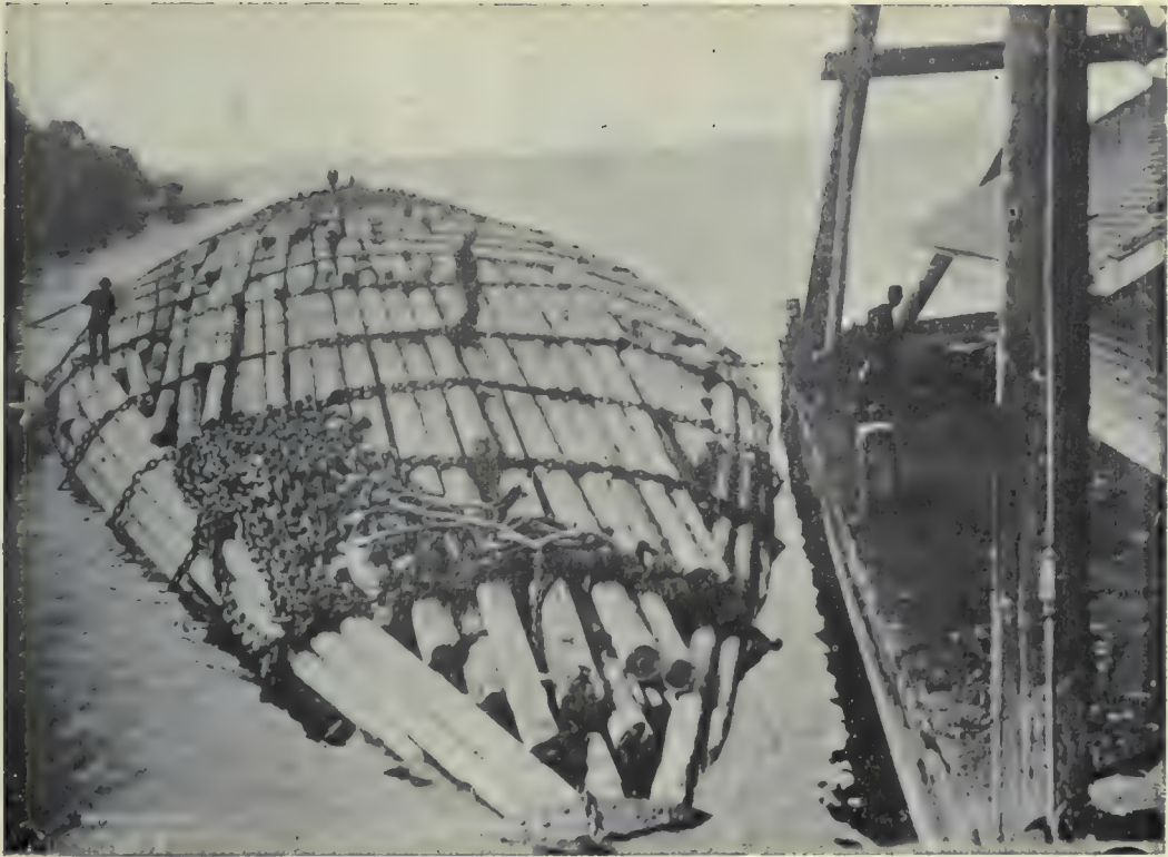
Benson Raft ready for sea, 8000 tons of logs, Length 1,000 ft.; Beam 60 ft.; Height 40 ft., (15 ft. above and 25 ft. below water) Photo by Gifford and Prentiss, Portland, Oregon.
