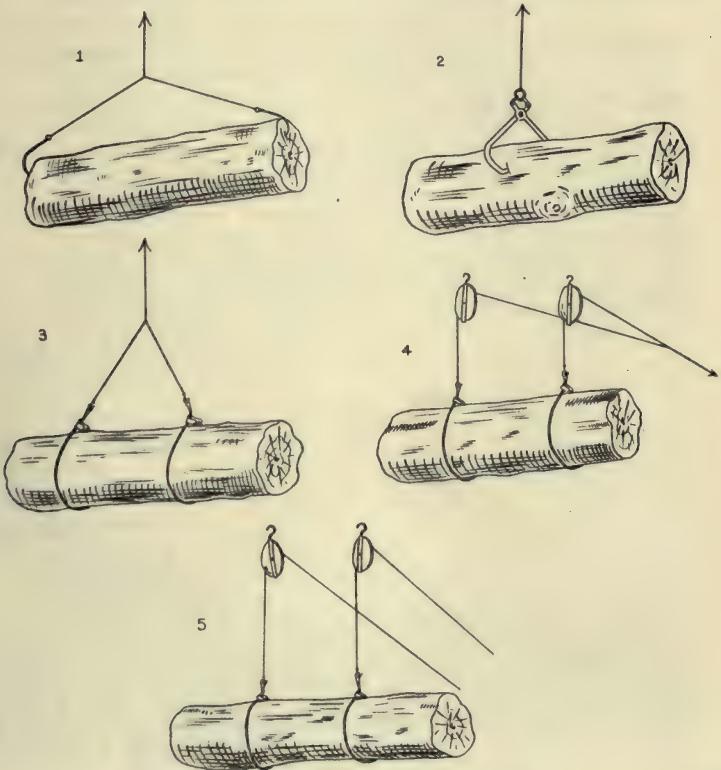
METHODS OF ATTACHMENT OF LOGS FOR LOADING.
