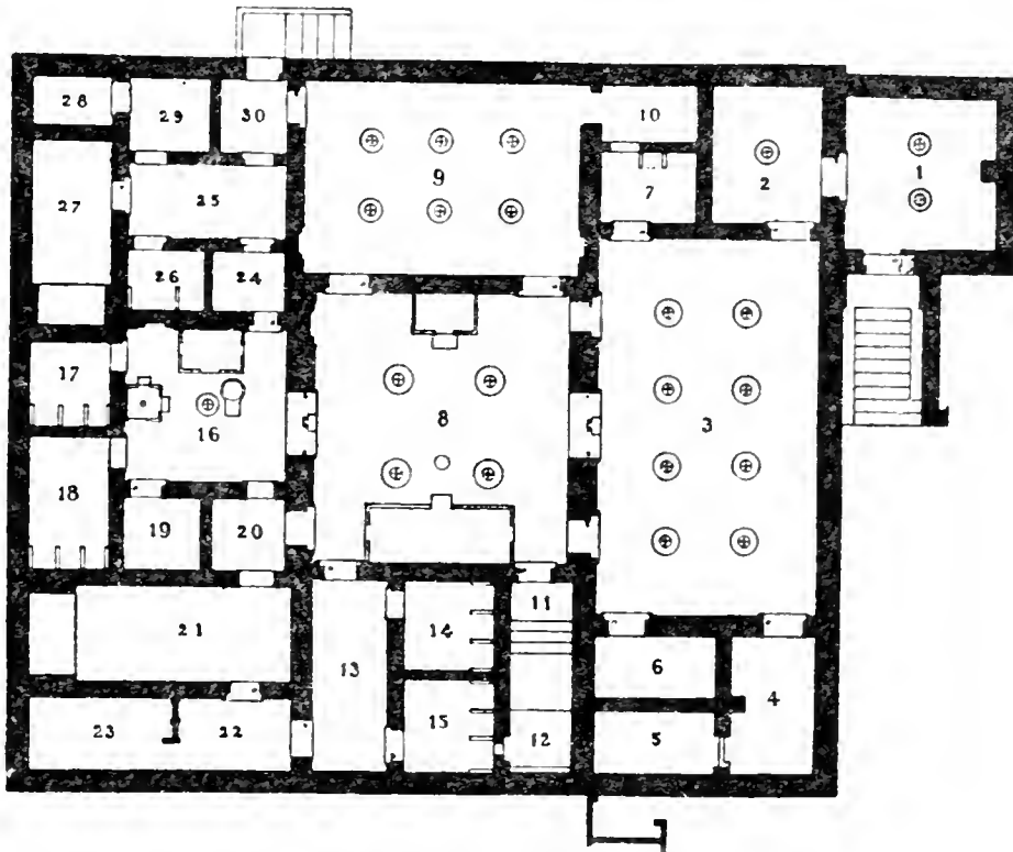
Fig. 2.—Ground Plan of a Mansion at El-Amarna.
