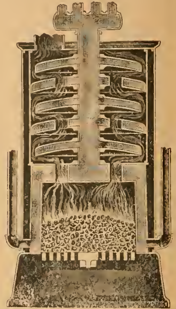
SWAMSCOT MACHINE CO.'S HOT WATER HEATER (PATENTED).
