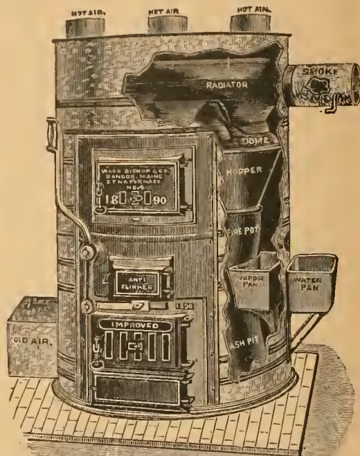
ETNA COAL FURNACE,
