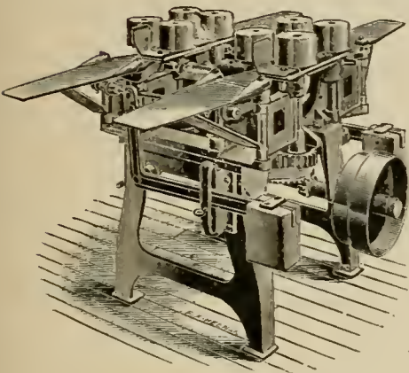
Box Matcher.
