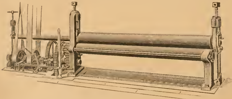
POWER BENDING ROLLS.
