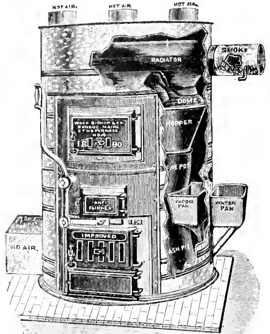
ETNA COAL FURNACE,
