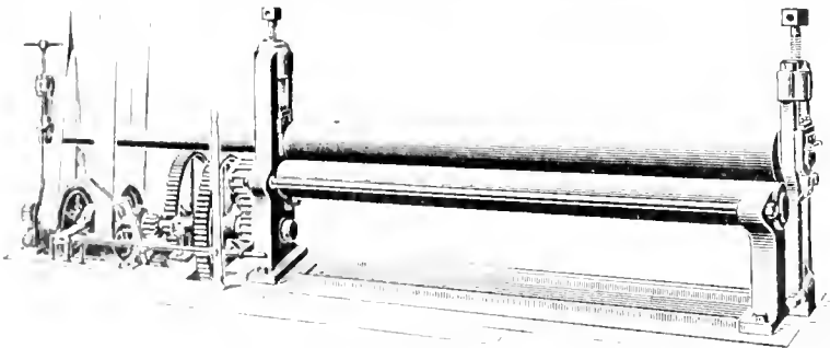
POWER BENDING ROLLS.
