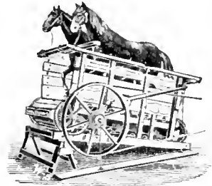
Horse Power.
