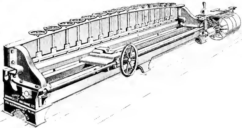
BOILER PLATE PLANER.
