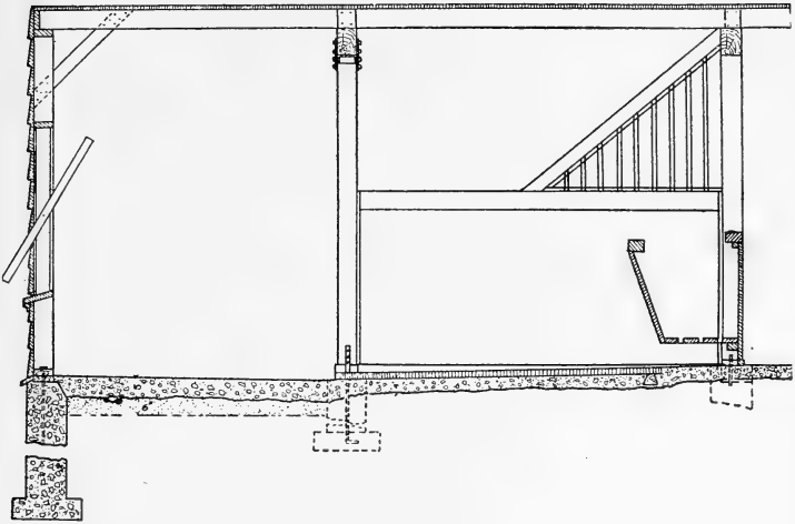
FIG. 180.—CROSS SECTION THROUGH HORSE BARN
