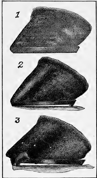
FIG. 165.—METHODS OF SHOEING 1, Normal position; 2, hasten the action; 3, retard the action.
